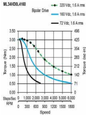
ML34HD0
