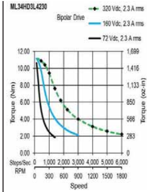
ML34HD3
