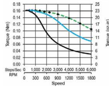
MS16HS4P6120 Unipolar Drive 36 Vdc, 1.2 A rms 24 Vdc, 1.2 A rms 12 Vdc, 1.2 A rms
