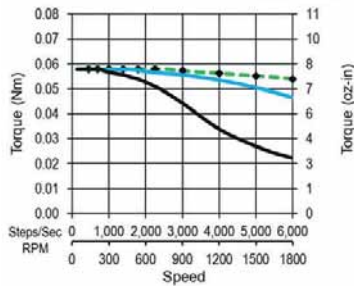
MS16HS7P6100 Unipolar Drive 36 Vdc, 1 A rms 24 Vdc, 1 A rms 12 Vdc, 1 A rms
