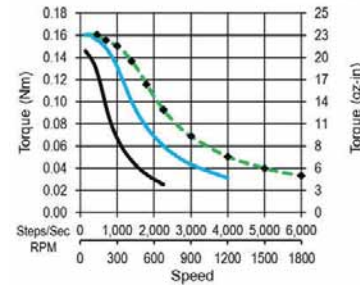
MS16HS4P6036 Unipolar Drive 36 Vdc, 0.36 A rms 24 Vdc, 0.36 A rms 12 Vdc, 0.32 A rms
