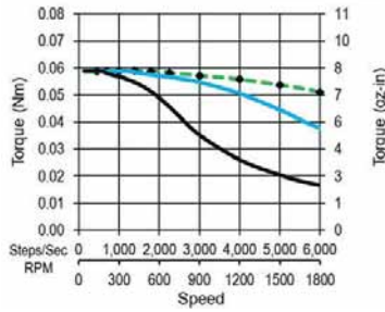
MS16HS7P6070 Unipolar Drive 36 Vdc, 0.7 A rms 24 Vdc, 0.7 A rms 12 Vdc, 0.7 A rms
