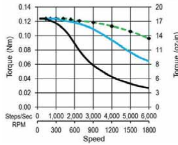
MS16HS0P6100 Unipolar Drive 36 Vdc, 1 A rms 24 Vdc, 1 A rms 12 Vdc, 1 A rms
