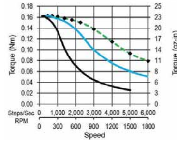
MS16HS4P6085 Unipolar Drive 36 Vdc, 0.85 A rms 24 Vdc, 0.85 A rms 12 Vdc, 0.85 A rms
