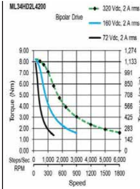
ML34HD2
