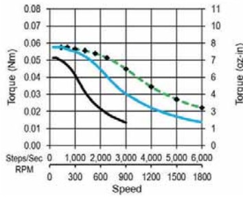
MS16HS7P6024 Unipolar Drive 36 Vdc, 0.24 A rms 24 Vdc, 0.24 A rms 12 Vdc, 0.21 A rms
