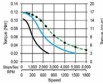
MS16HS0P6027 Unipolar Drive 36 Vdc, 0.27 A rms 24 Vdc, 0.27 A rms 12 Vdc, 0.23 A rms
