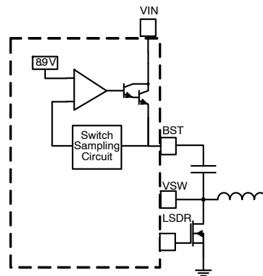
Figure 29. Boost Circuit
