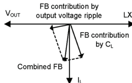
Fig. 17 - FB Voltage in Phasor Diagram
