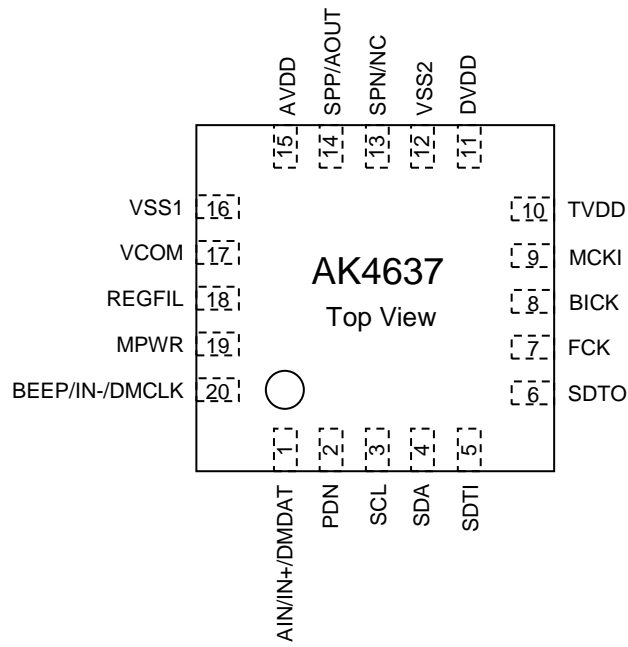
Figure 2. Pin Layout
