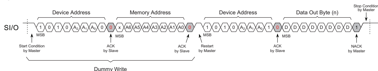
Figure 8-2. Random Read
