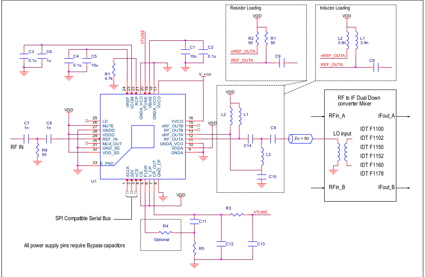
Figure 13B. Schematic Example for Driving Single Ended Mixer
