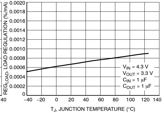
Figure 12. Load Regulation vs. Temperature – V OUT = 3.3 V
