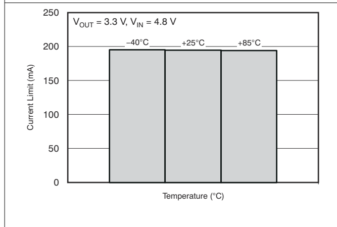
Figure 6-17. Current Limit vs Junction Temperature for Legacy Chip
