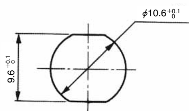
Type HR10A-10WTR (Panel thickness 1 to 2mm)
