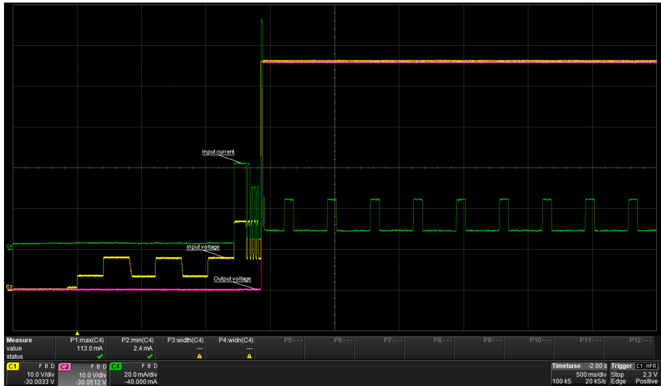
Figure 17. No Load Start-up, MPS Circuit Turned ON
