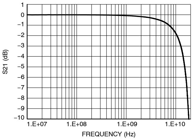
Figure 5. Insertion Loss
