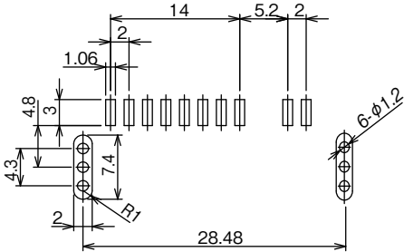
Recommended PCB Dimensions
