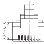
FCC Plug Dimensions
