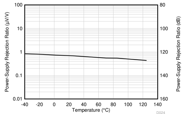
Figure 6-24. PSRR vs Temperature
