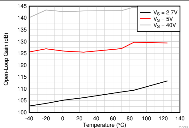
Figure 6-29. Open-Loop Voltage Gain vs Temperature (dB)
