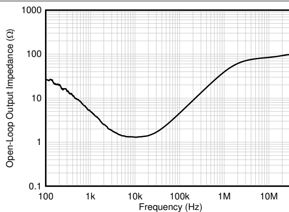
Figure 6-30. Open-Loop Output Impedance vs Frequency
