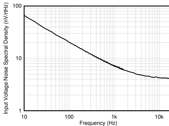
Figure 6-26. Input Voltage Noise Spectral Density vs Frequency
