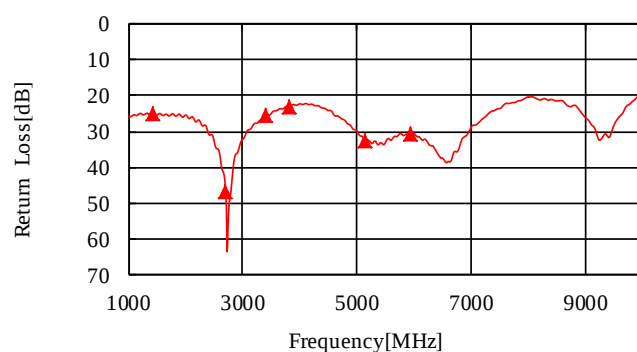
S11(Main Line)
