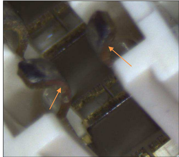
Bottom View, Scratches on sides of contact legs
