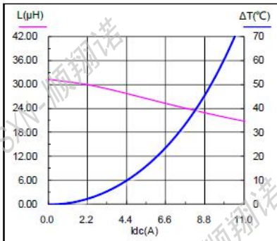
SMMS1770-330M
