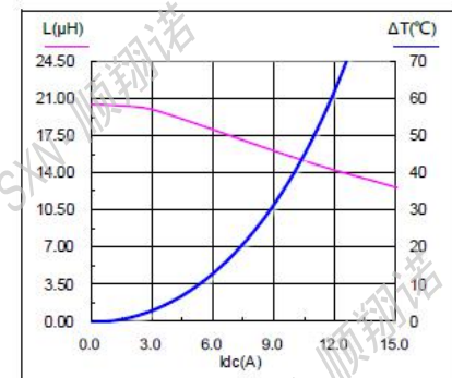
SMMS1770-680M
