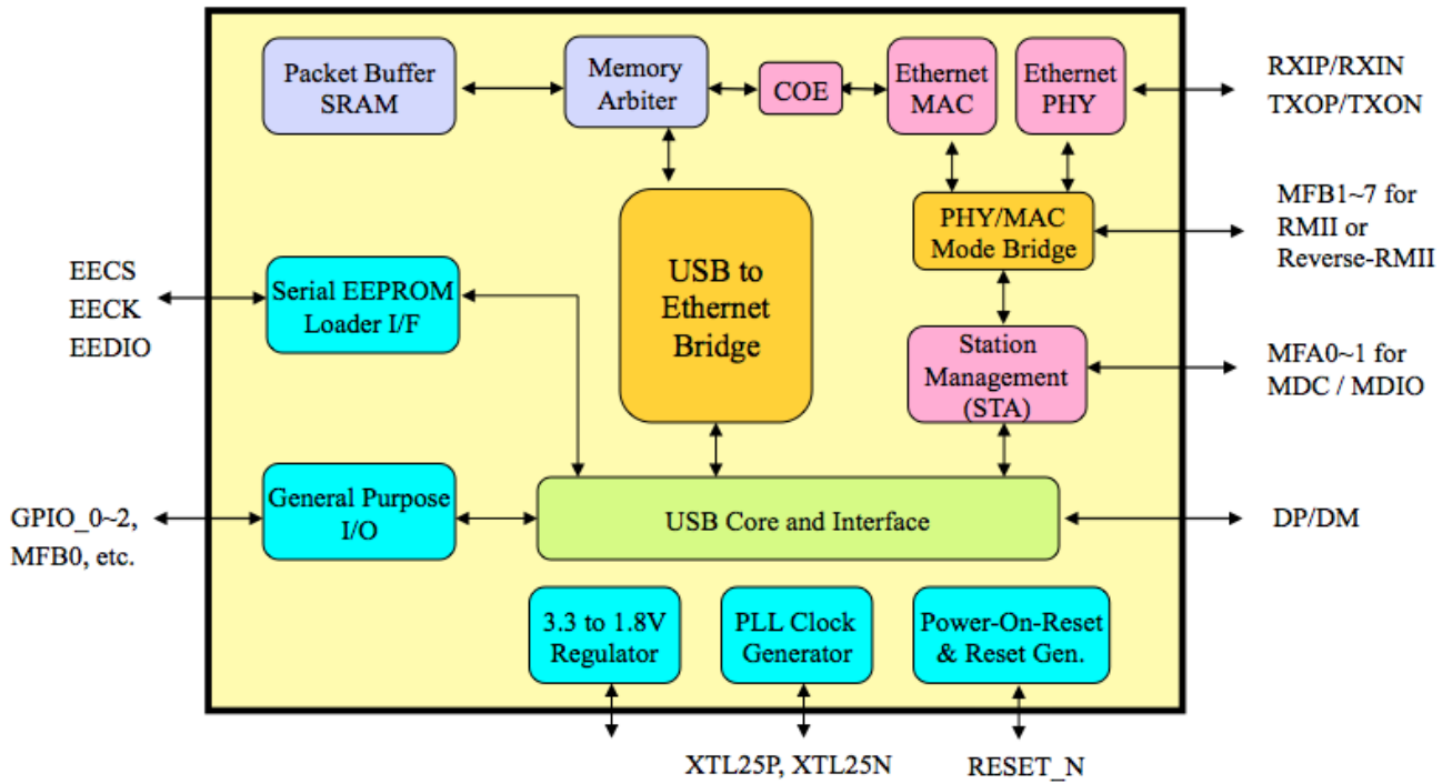
Figure 1. Block Diagram
