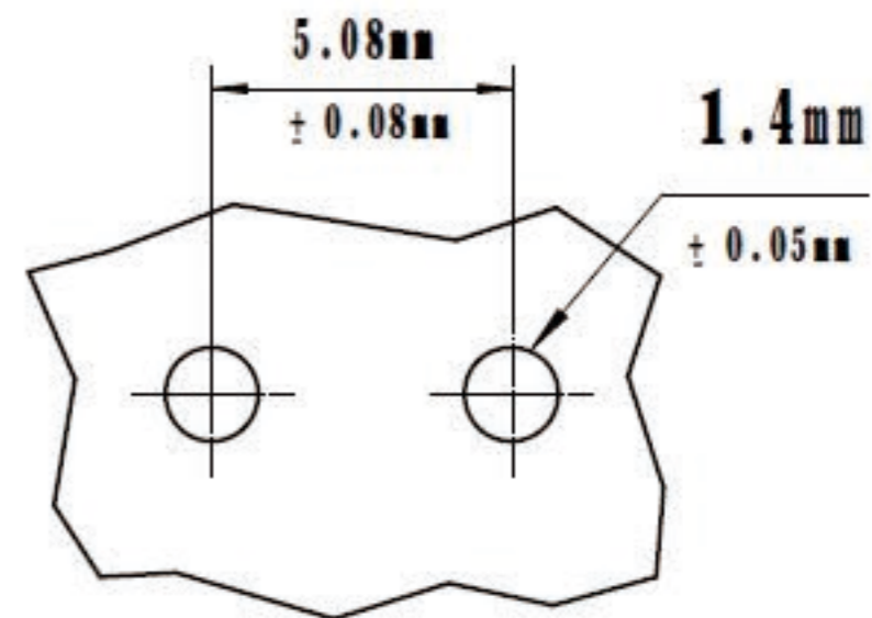
P.C. BOARD HOLE PATTERN
