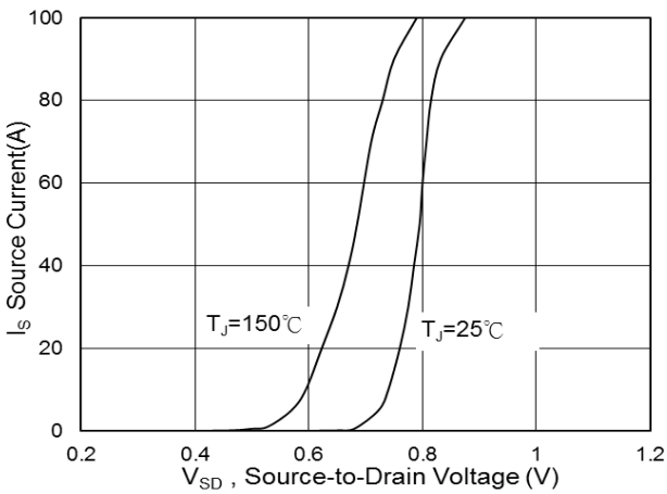
Fig.3 Diode Forward Voltage vs. Current
