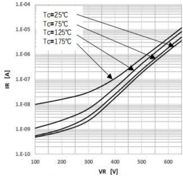
Figure 2 Reverse Characteristics
