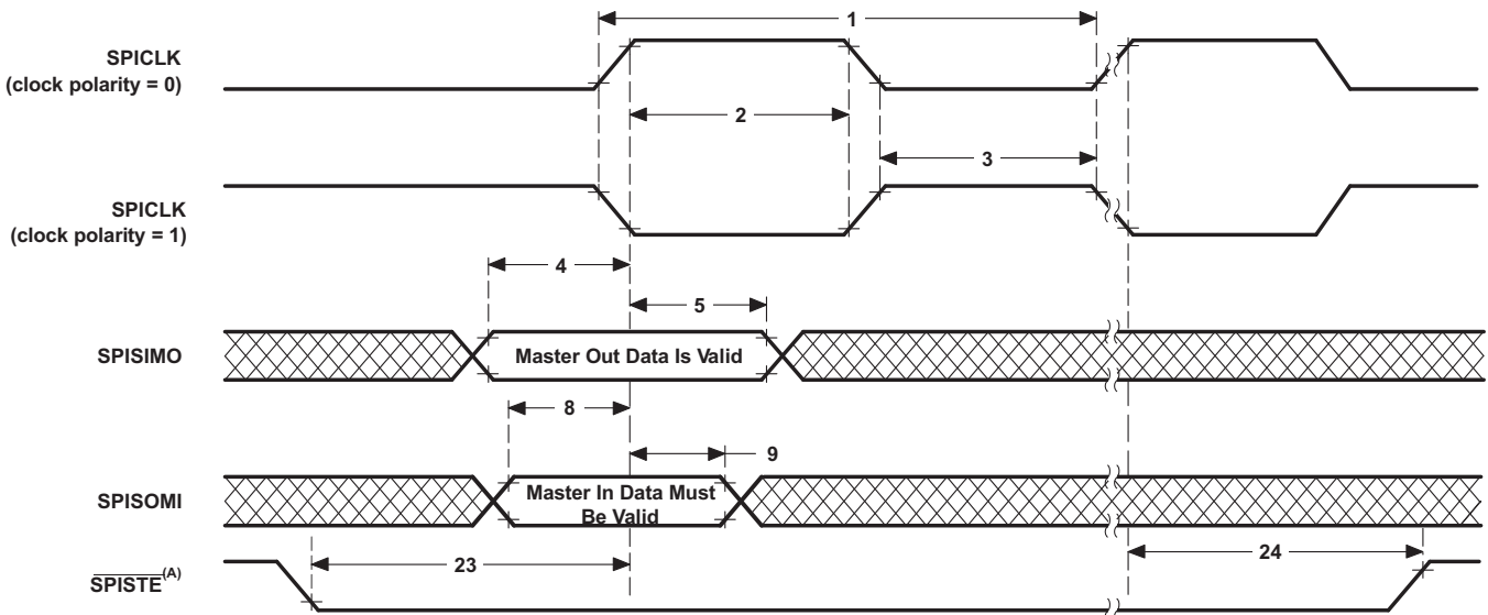
Figure 5-70. High-Speed SPI Master Mode External Timing (Clock Phase = 0)
