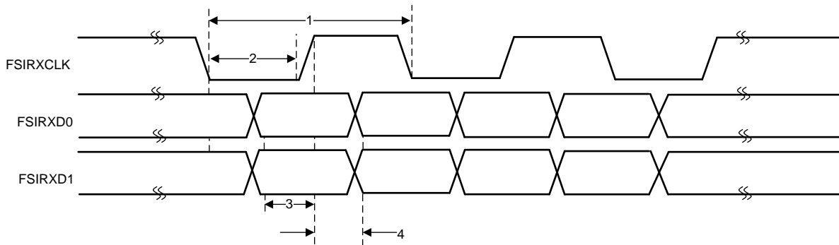
Figure 5-80. FSIRX Timings
