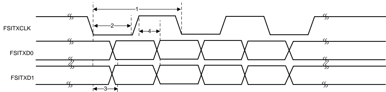
Figure 5-77. FSITX Timings
