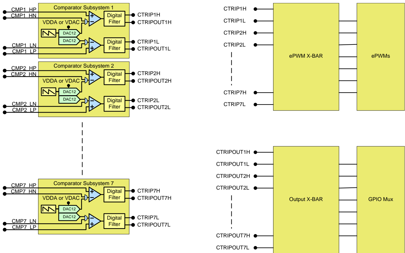
Figure 5-40. CMPSS Connectivity
