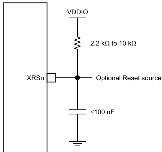
Figure 5-6. Reset Circuit
