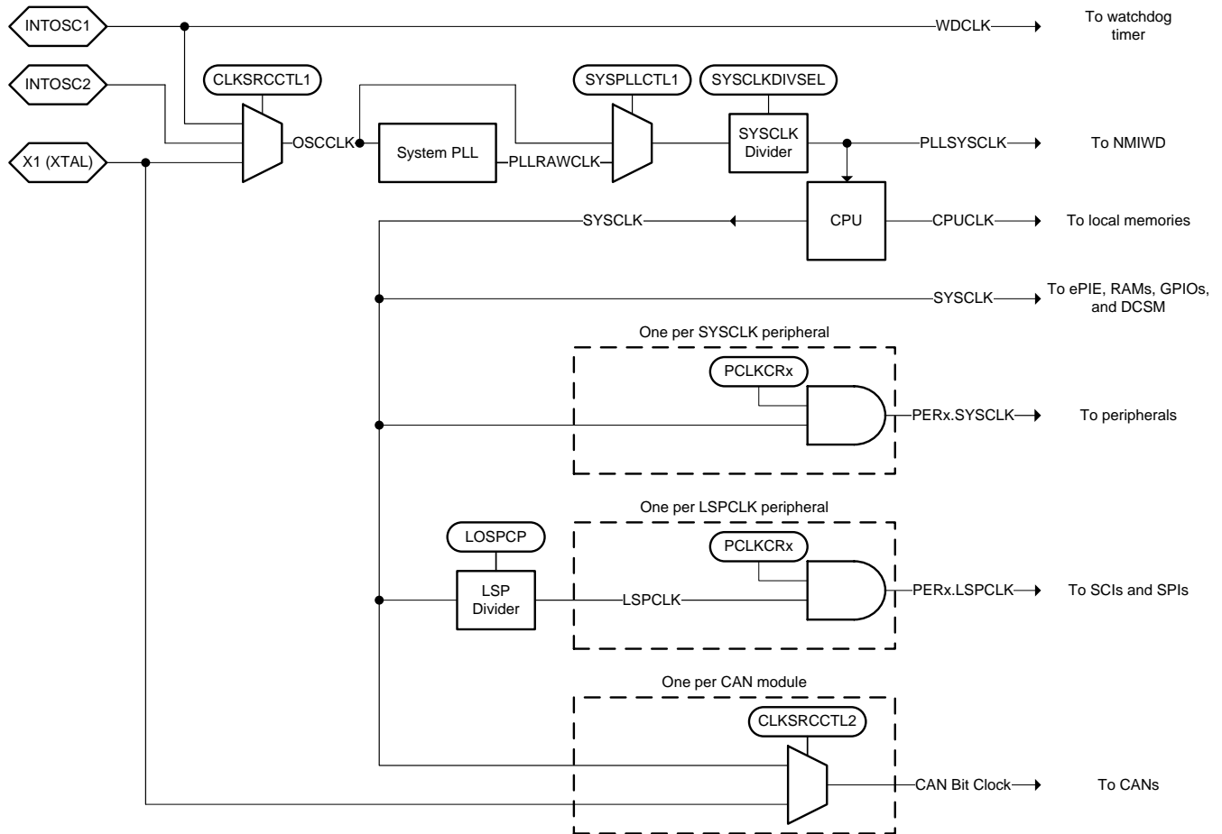
Figure 5-9. Clocking System
