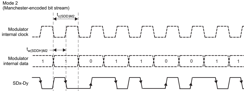
Figure 5-59. SDFM Timing Diagram – Mode 2
