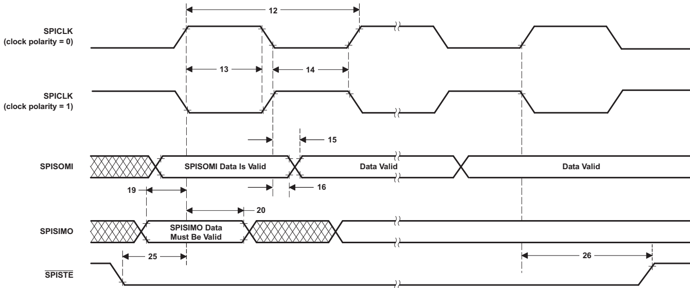
Figure 5-73. High-Speed SPI Slave Mode External Timing (Clock Phase = 1)
