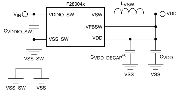
Figure 5-5. DC-DC Circuit Schematic
