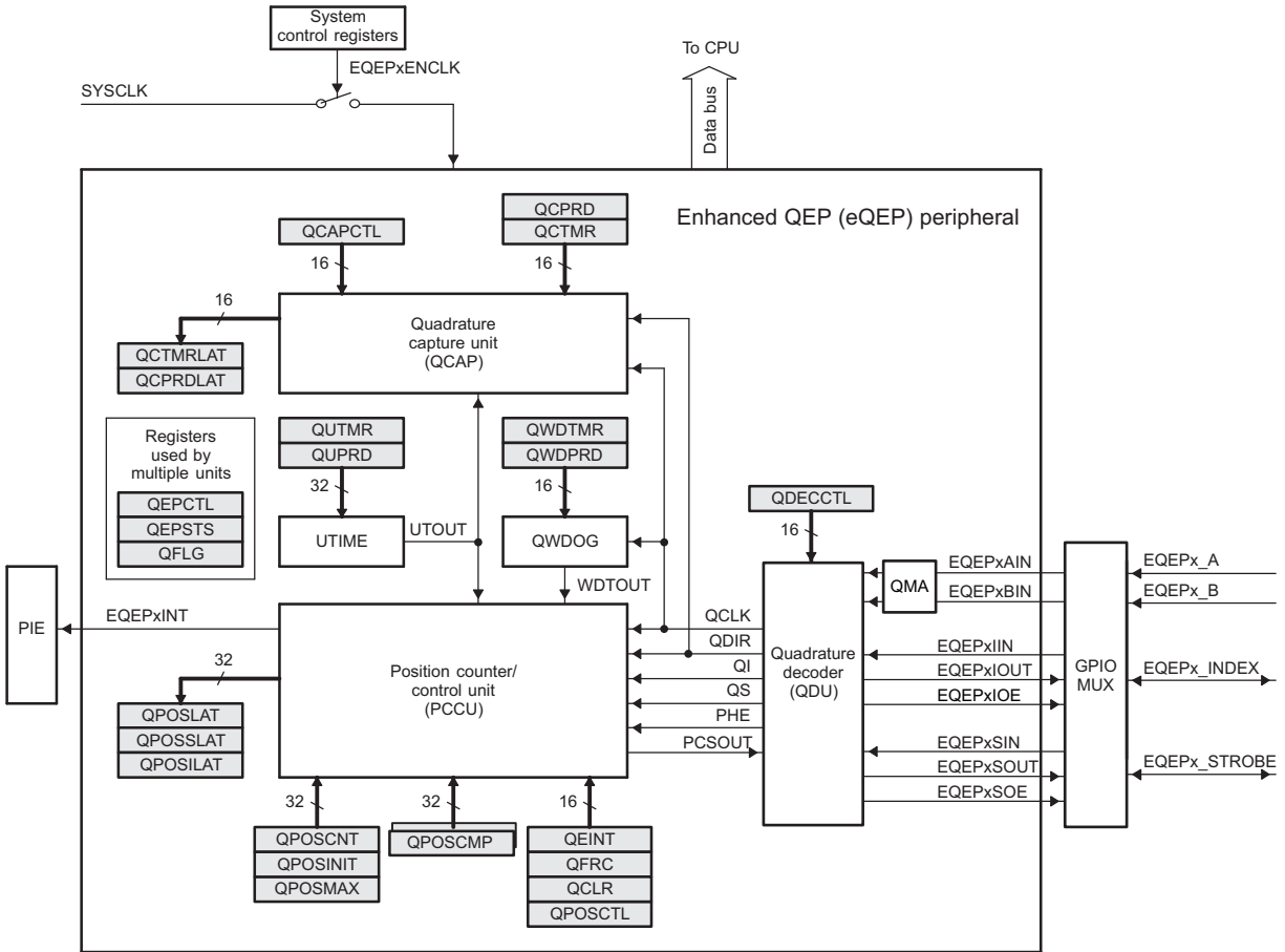
Figure 5-55. eQEP Block Diagram
