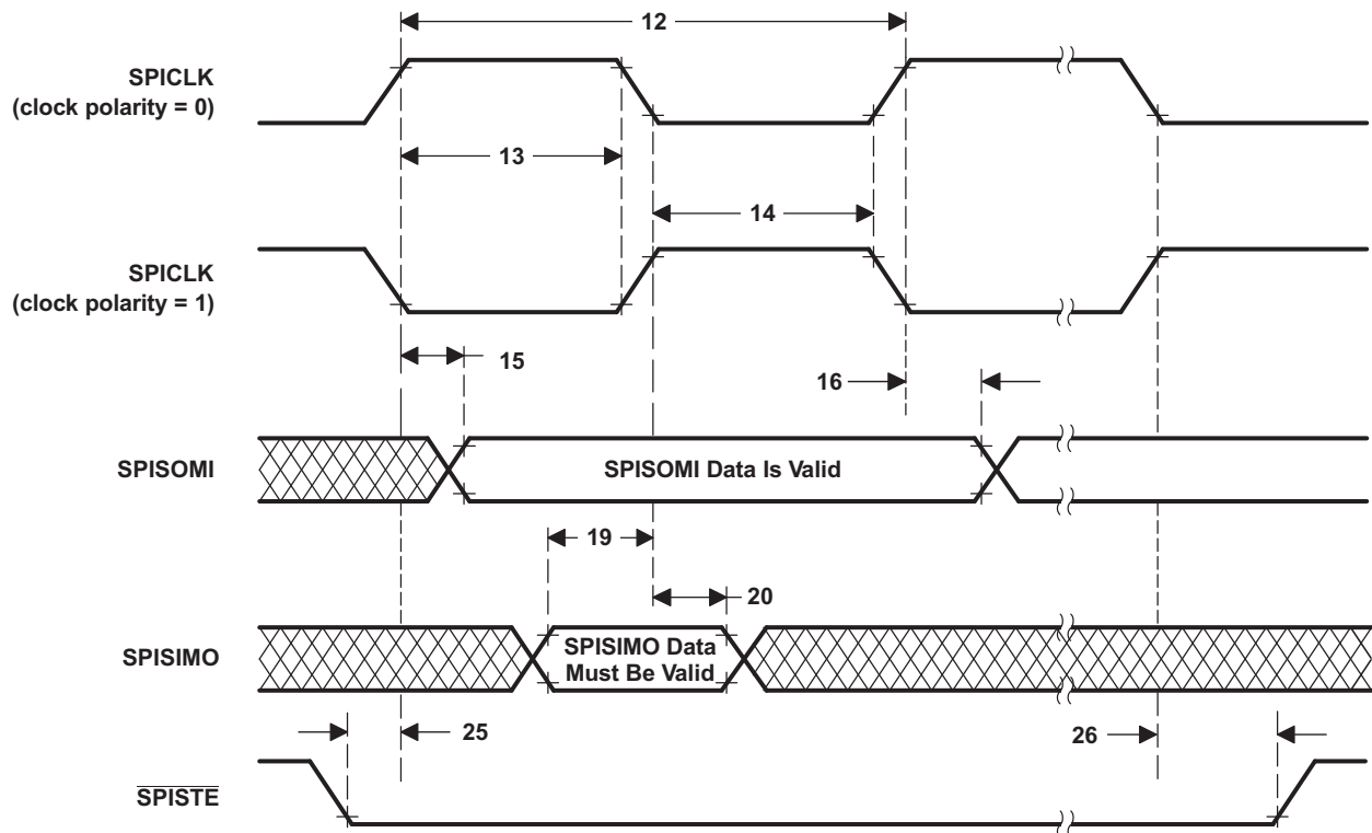
Figure 5-68. SPI Slave Mode External Timing (Clock Phase = 0)
