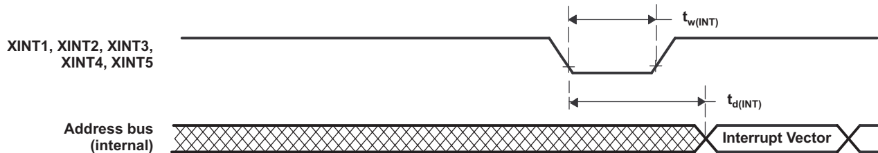
Figure 5-24. External Interrupt Timing
