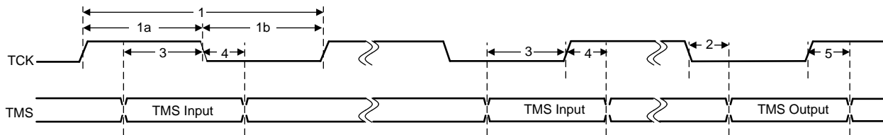
Figure 5-19. cJTAG Timing
