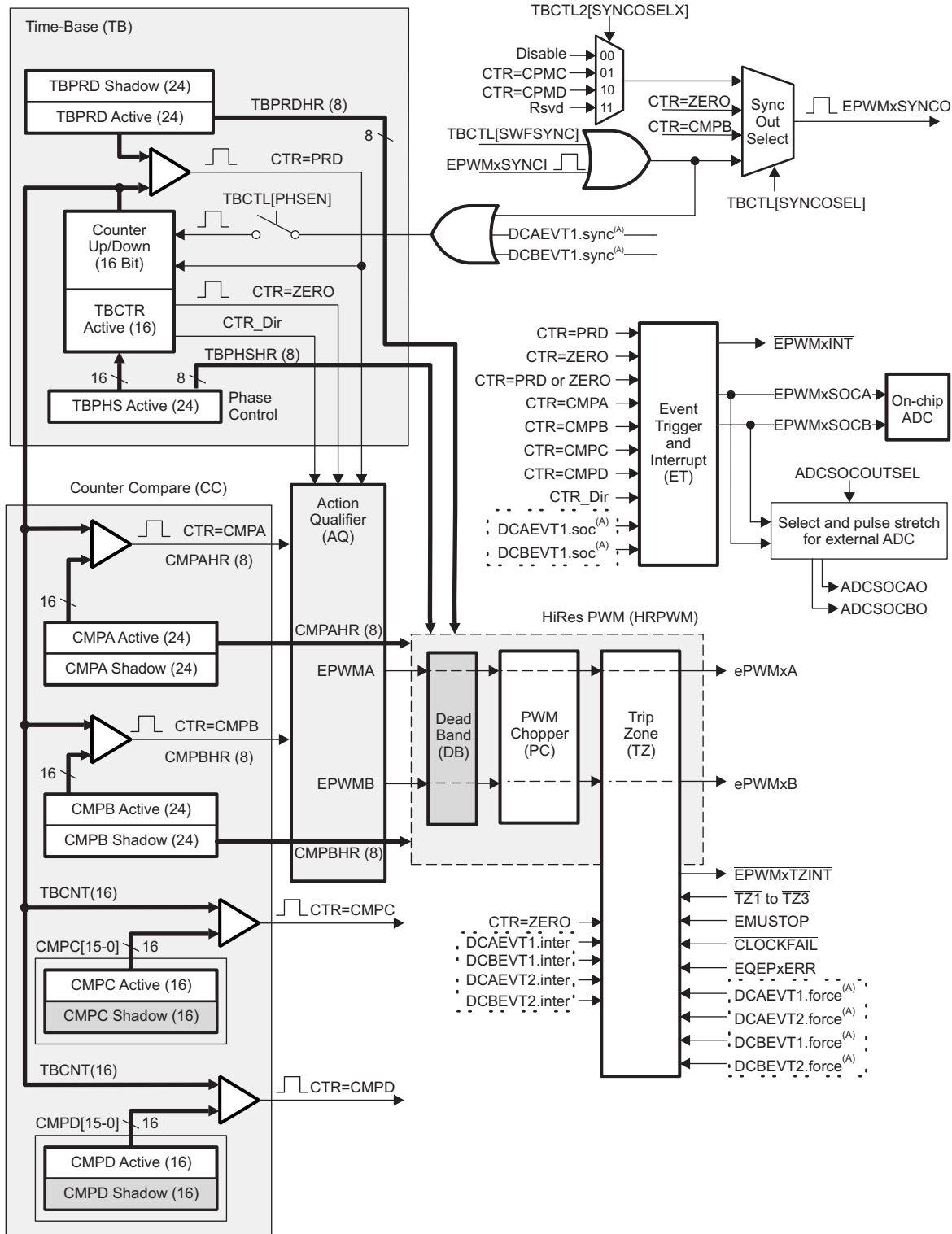
Figure 5-50. ePWM Submodules and Critical Internal Signal Interconnects
