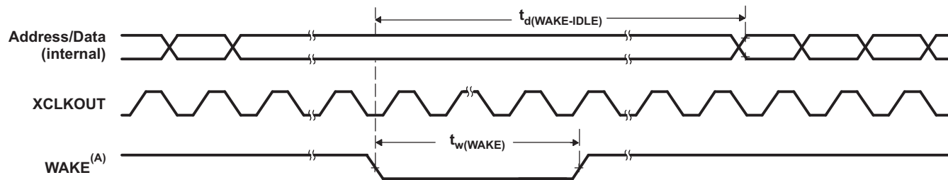
Figure 5-25. IDLE Entry and Exit Timing Diagram
