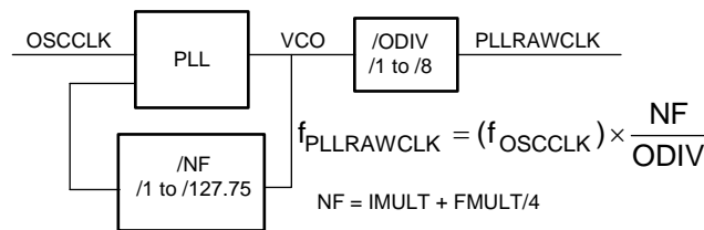
Figure 5-10. System PLL
