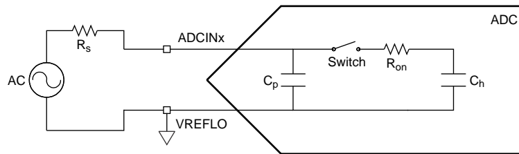
Figure 5-33. Input Model
