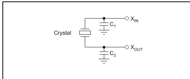
Figure 6. Crystal Connection.
