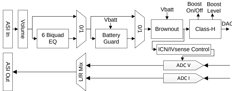
图 37. ROM Mode 1 Processing Block Diagram
