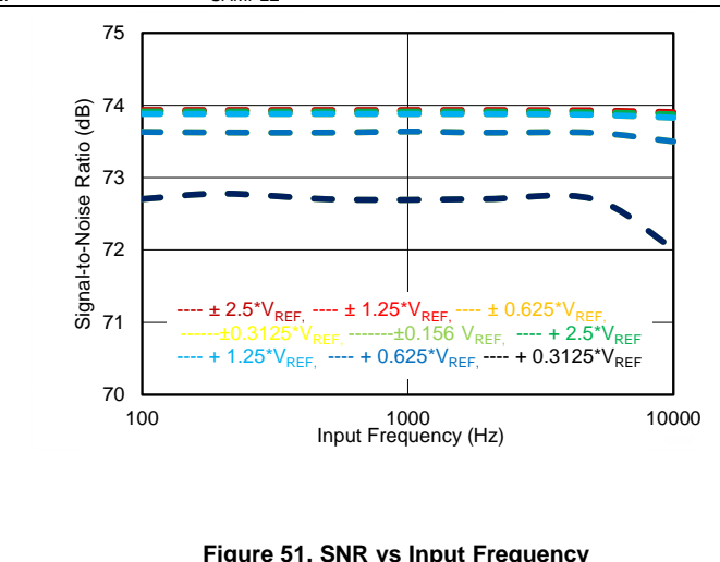
Figure 51. SNR vs Input Frequency
