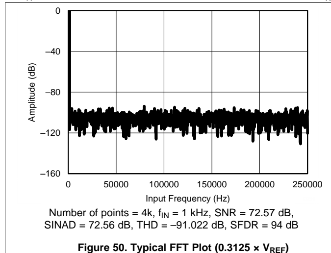
Figure 50. Typical FFT Plot ( 0.3125 \times V_{REF} )
