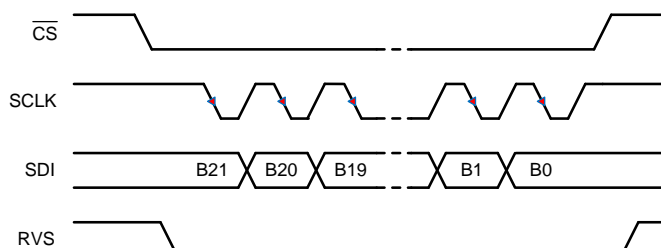
Figure 49. SPI-10-S Protocol, Optimal Command Frame
