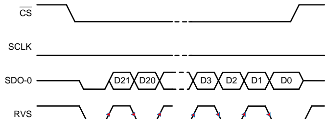
Figure 73. SRC-INT-SD: SRC, INTCLK, Single SDO, DDR
