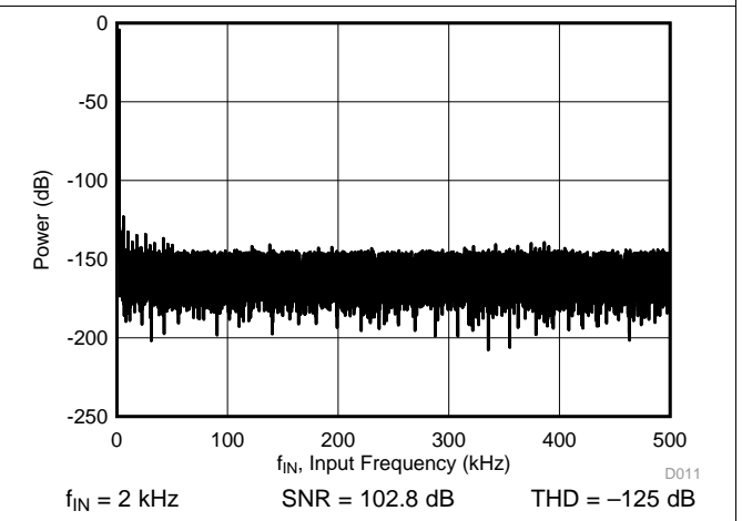
Figure 21. Typical FFT
