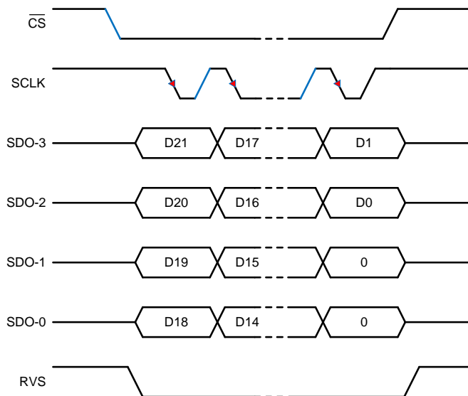
Figure 63. SPI-10-Q Protocol
