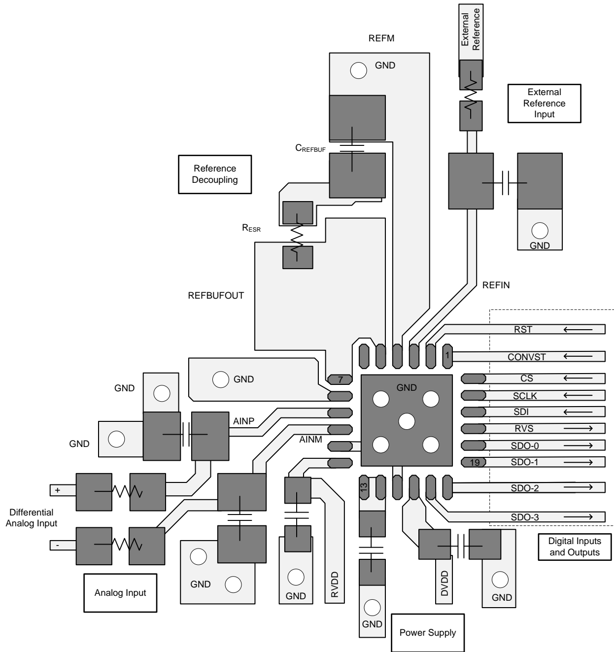
Figure 104. Recommended Layout
