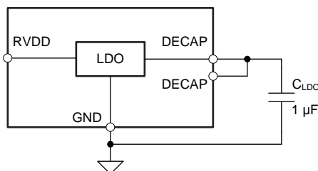
Figure 28. Internal LDO Connections
