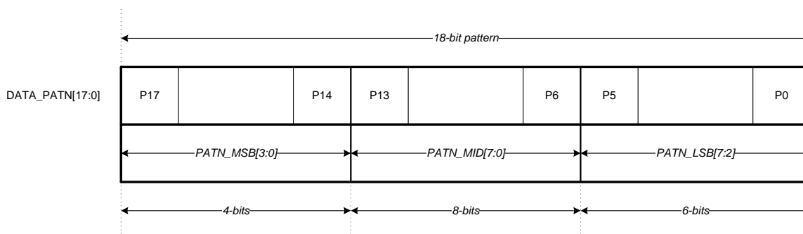
Figure 96. DATA_PATN[17:0]
