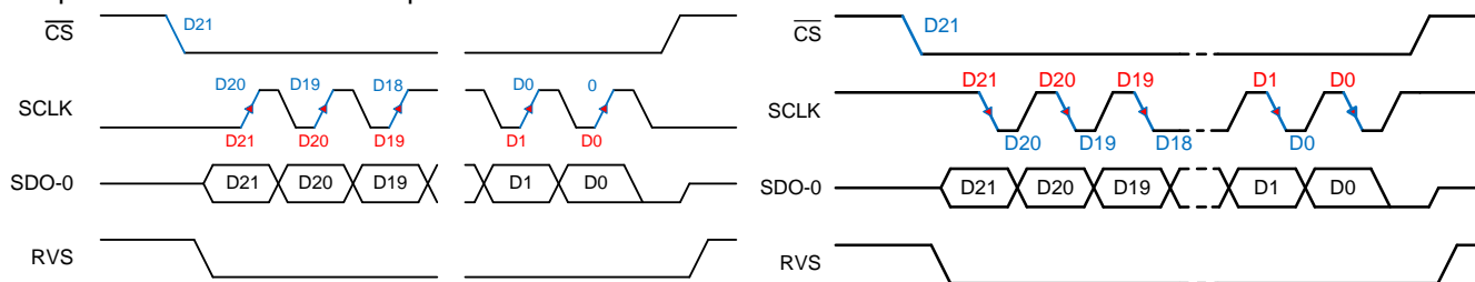
Figure 55. SPI-00-S-EDL Protocol, 22 SCLKs
