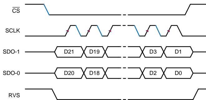
Figure 57. SPI-00-D Protocol
