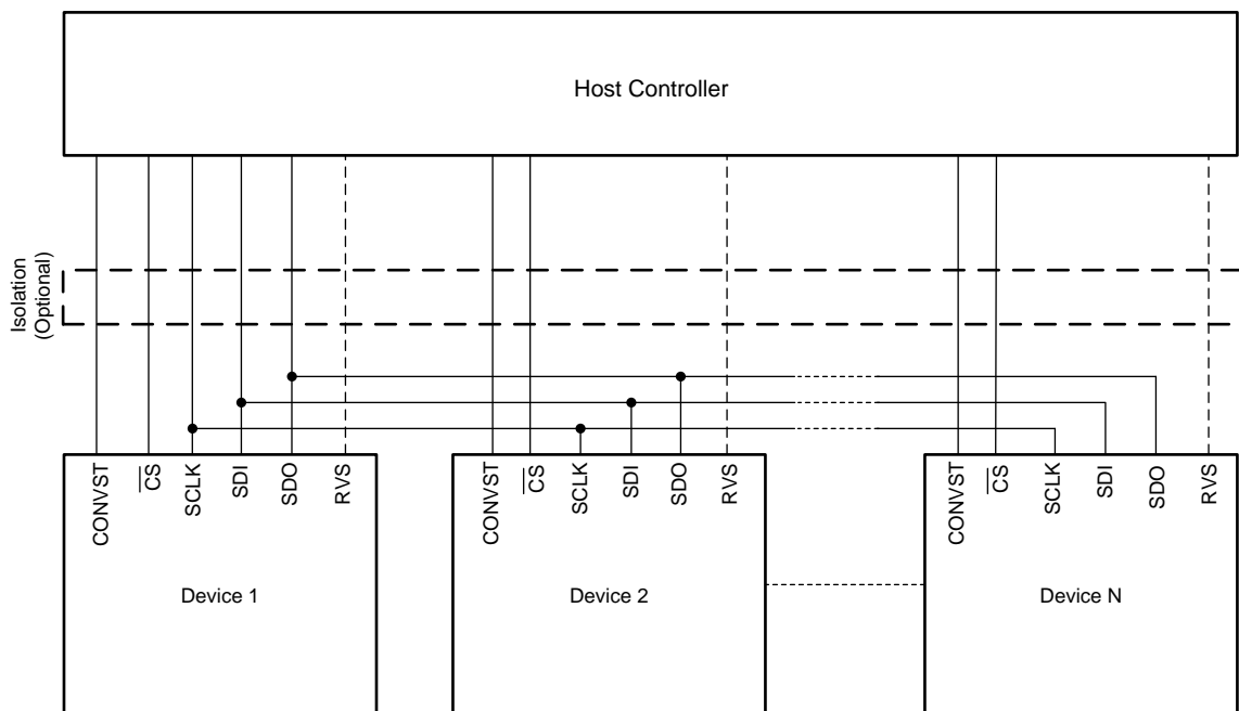
Figure 87. Star-Topology Connection
