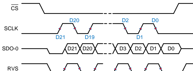
Figure 72. SRC-EXT-SD: SRC, SCLK, Single SDO, DDR
