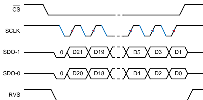
Figure 60. SPI-11-D Protocol
