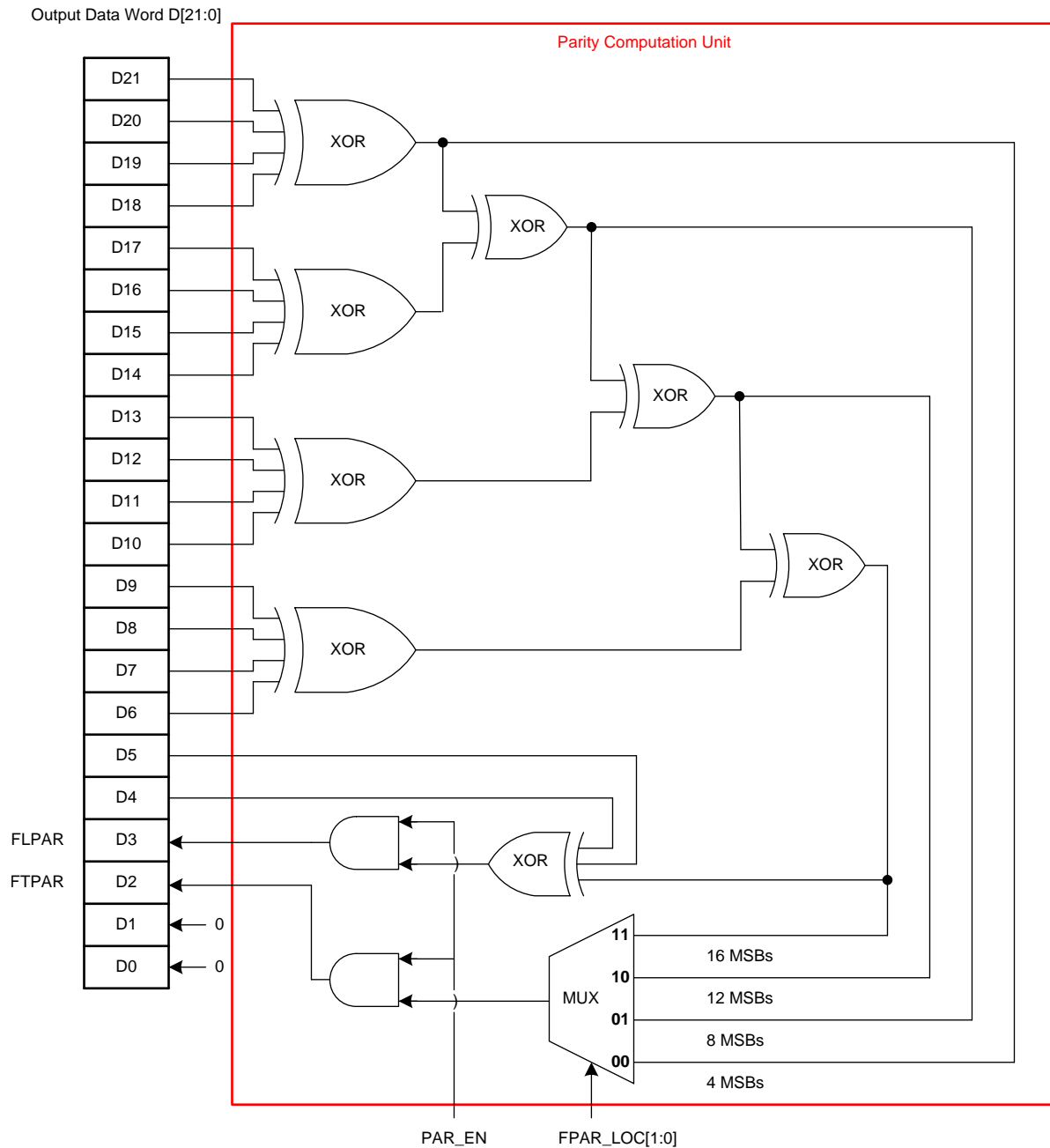
Figure 39. Parity Bits Computation
