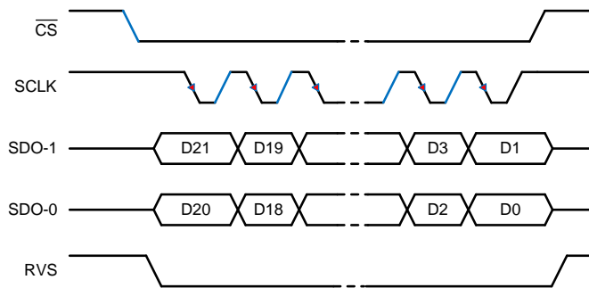
Figure 59. SPI-10-D Protocol
