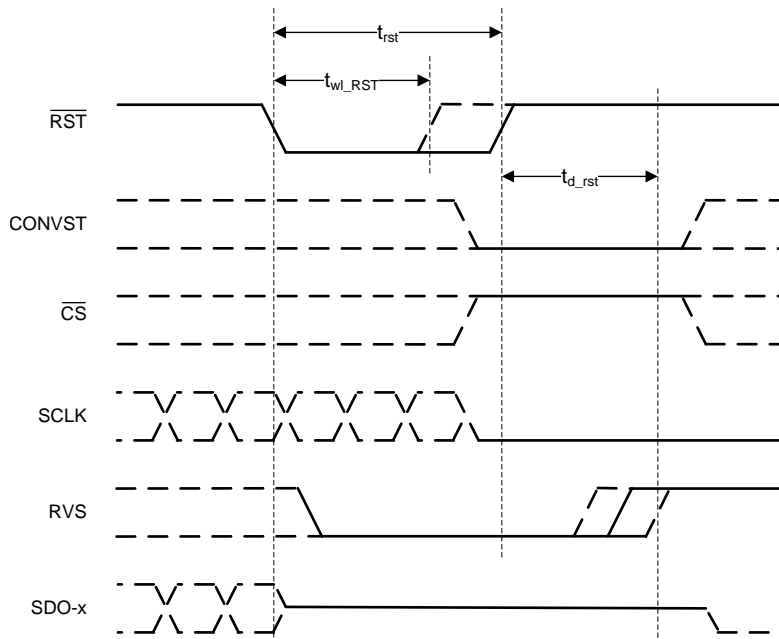
Figure 36. Asynchronous Reset
