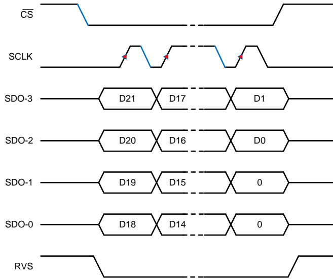
Figure 61. SPI-00-Q Protocol
