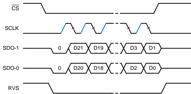
Figure 58. SPI-01-D Protocol
