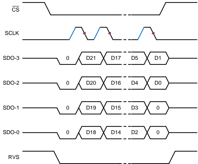
Figure 62. SPI-01-Q Protocol
