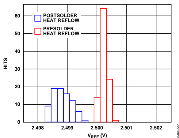
图55. SHR基准电压偏移
