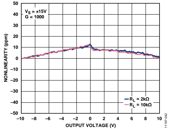
Figure 39. Gain Nonlinearity (G = 1000)
