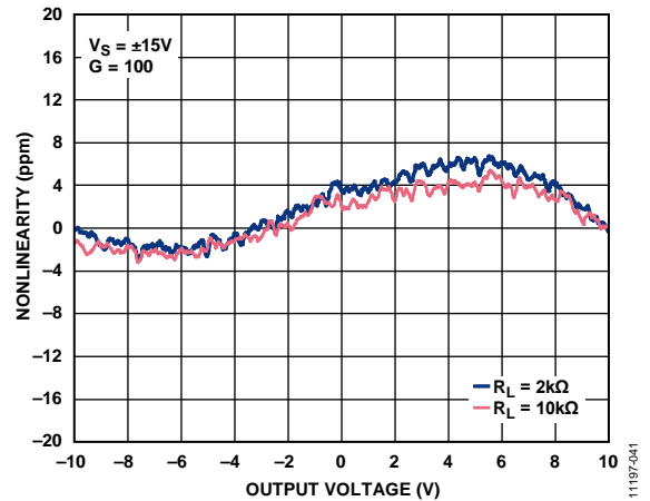
Figure 38. Gain Nonlinearity (G = 100)
