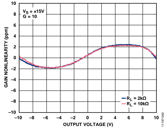
Figure 37. Gain Nonlinearity (G = 10)
