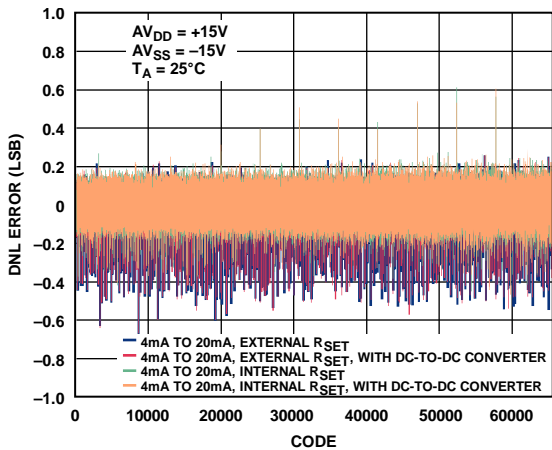
Figure 33. Differential Nonlinearity vs. Code
