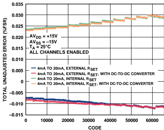
Figure 34. Total Unadjusted Error vs. Code
