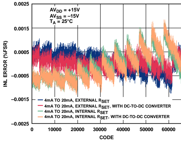
Figure 32. Integral Nonlinearity vs. Code
