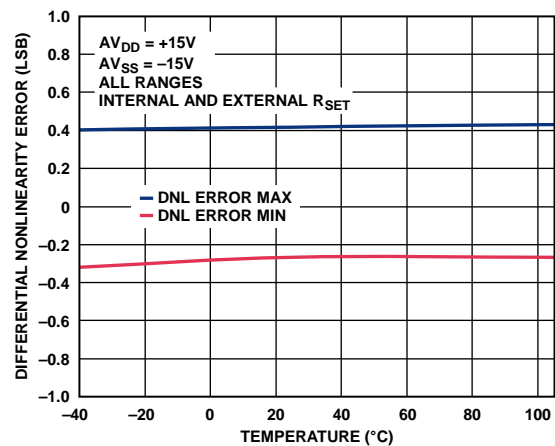
Figure 37. Differential Nonlinearity vs. Temperature
