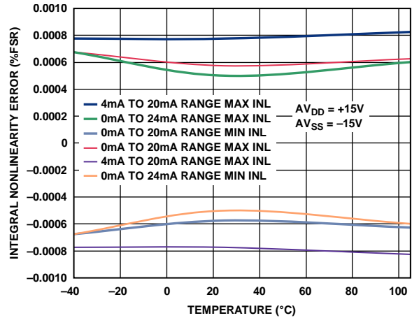
Figure 35. Integral Nonlinearity vs. Temperature, Internal RSET
