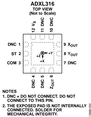
Figure 2. Pin Configuration
