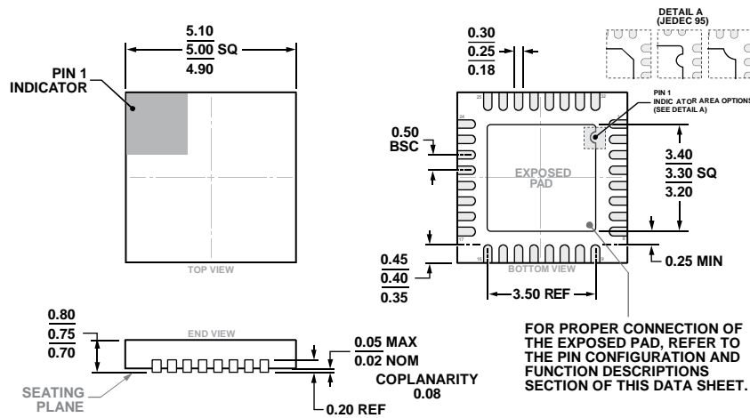
Figure 65. 32-Lead Lead Frame Chip Scale Package [LFCSP] 5 mm × 5 mm Body and 0.75 mm Package Height (CP-32-20)
