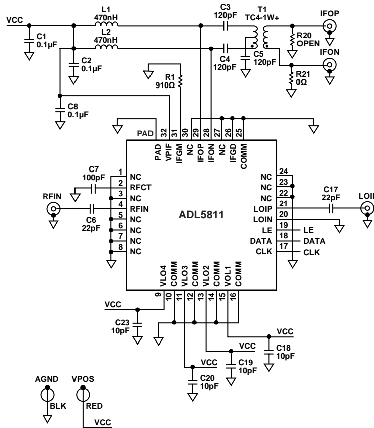
Figure 59. Basic Connections
