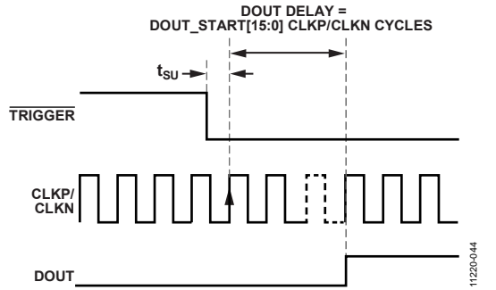
Figure 44. DOUT Start Sequence
