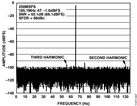
图7. 单音FFT( f_{IN} = 185.1\text{ MHz} )
