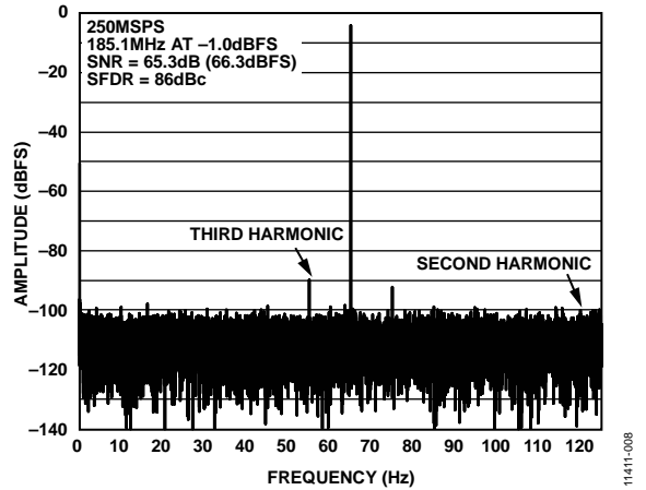
图8. 单音FFT( f_{IN} = 185.1\text{ MHz} , RFCLK = 1.0\text{ GHz} , 4分频(地址0x09 = 0x21))
