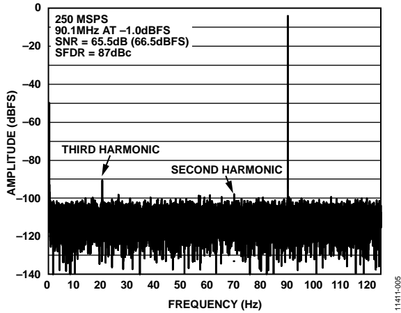
图5. 单音FFT( f_{IN} = 90.1\text{ MHz} )
