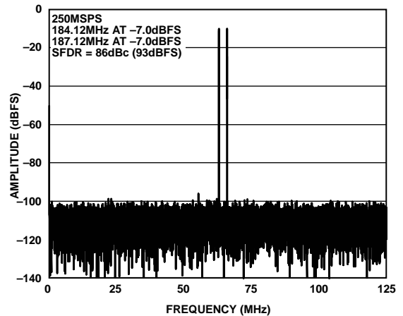
图16. 双音FFT( f_{IN1} = 184.12 MHz, f_{IN2} = 187.12 MHz)
