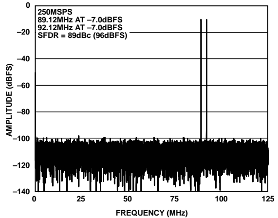
图15. 双音FFT( f_{IN1} = 89.12 MHz, f_{IN2} = 92.12 MHz)
