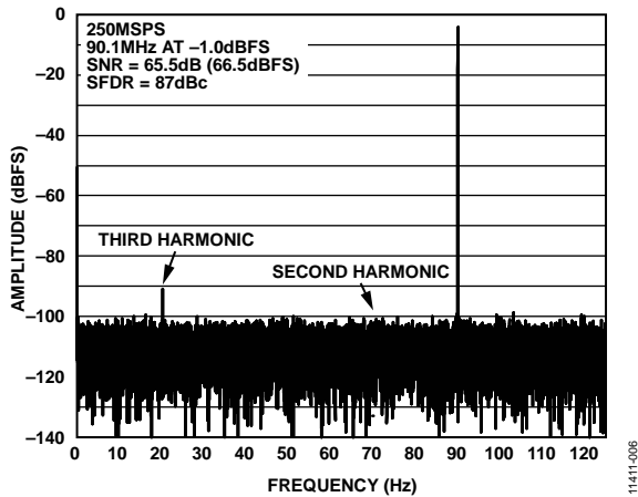
图6. 单音FFT( f_{IN} = 90.1\text{ MHz} , RFCLK = 1.0\text{ GHz} , 4分频(地址0x09 = 0x21))
