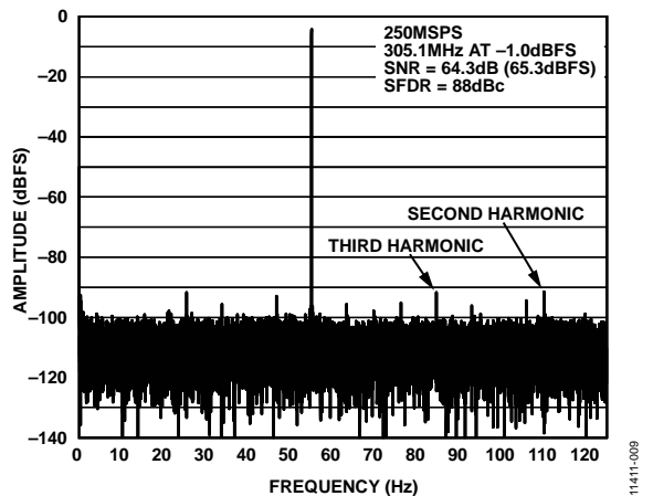
图9. 单音FFT( f_{IN} = 305.1\text{ MHz} )
