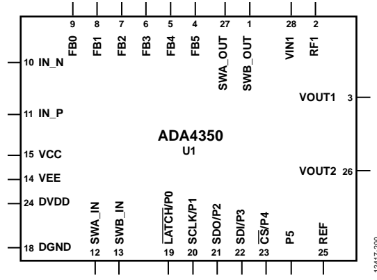
Figure 56. Recommended Symbol Layout
