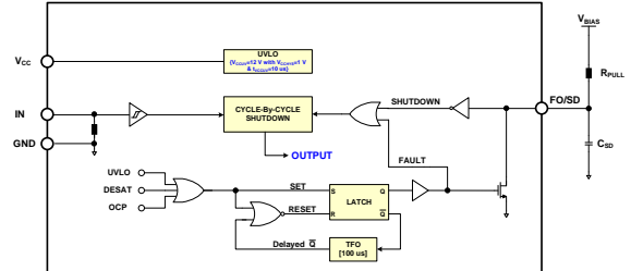
Figure 43. Application Circuit of Fault-Out
