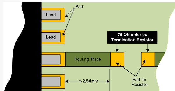
Figure 20. Termination Resistor Placement
