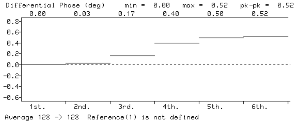
Figure 8. Differential Phase
