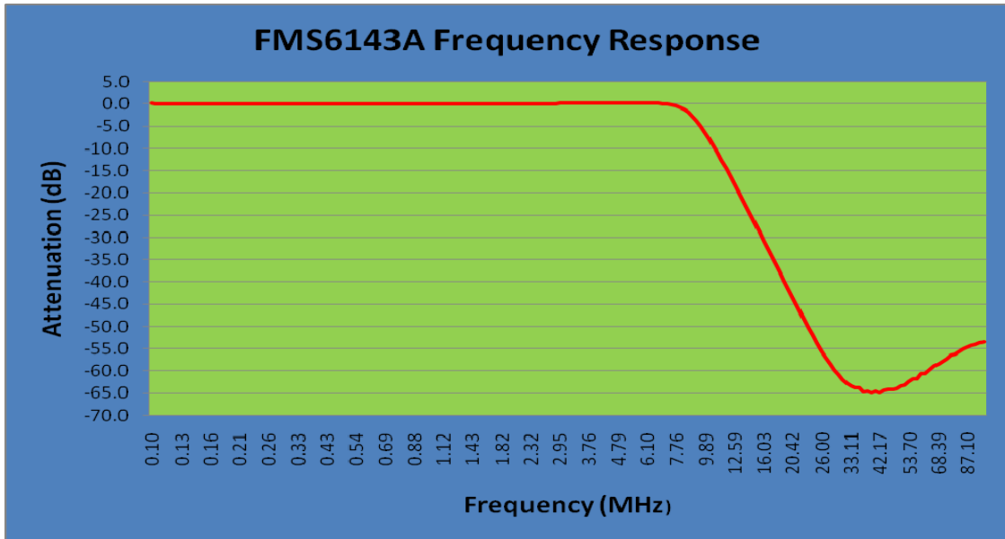
Figure 3. Frequency Response
