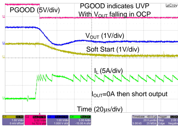
Figure 23. Over-Current Protection with Heavy Load Applied
