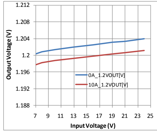
Figure 12. Line Regulation
