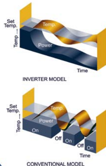
Fig. 9: Inverter control vs. conventional control
