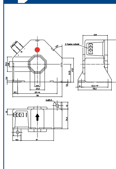
LA 305-S/SP5
