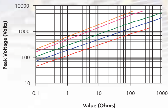
WA80 Series 1.2/50 \mu s Graph
