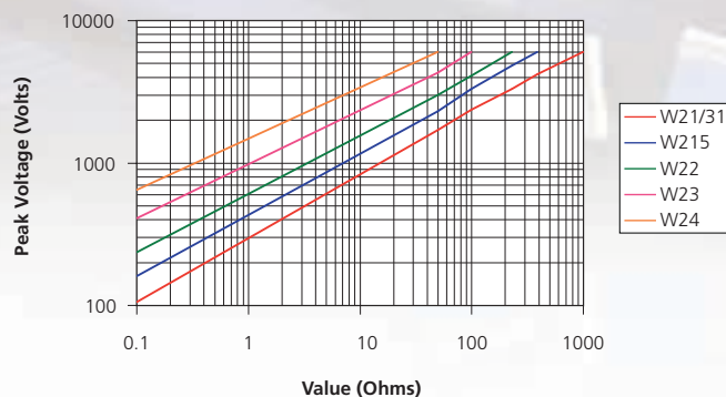
W21 Series & W31 1.2/50 \mu s Graph
