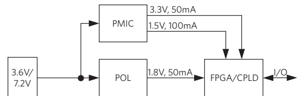
Figure 2. Typical FPGA Power Architecture Used in Communications, Industrial, and Consumer Applications
