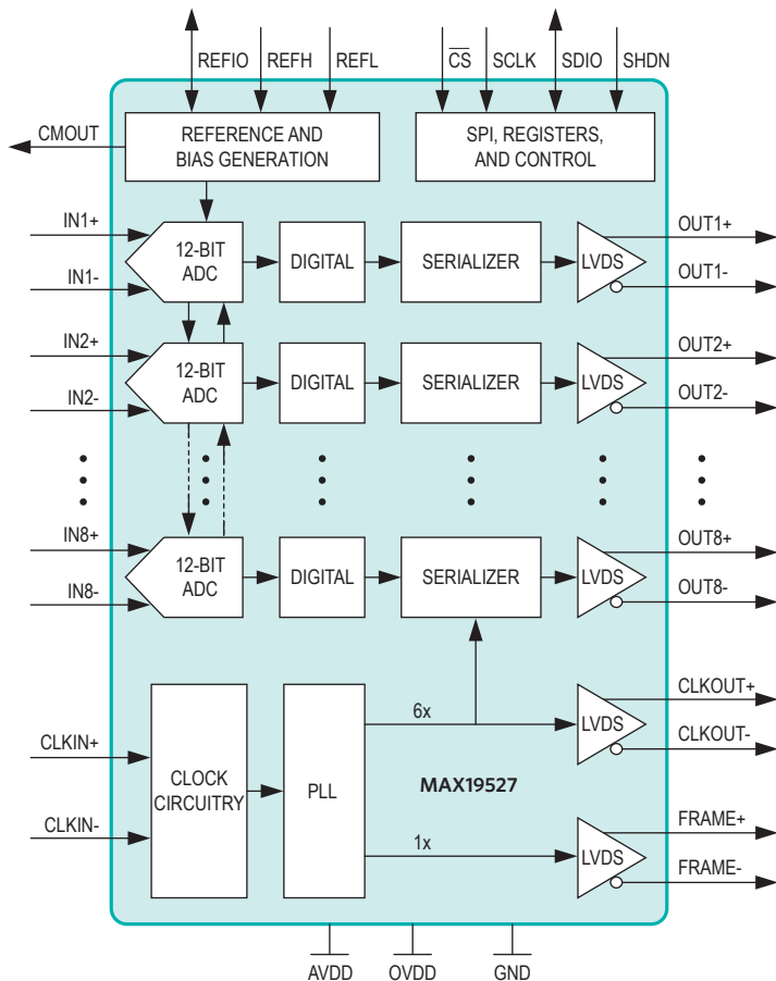
Figure 18. MAX19527 Functional Diagram
