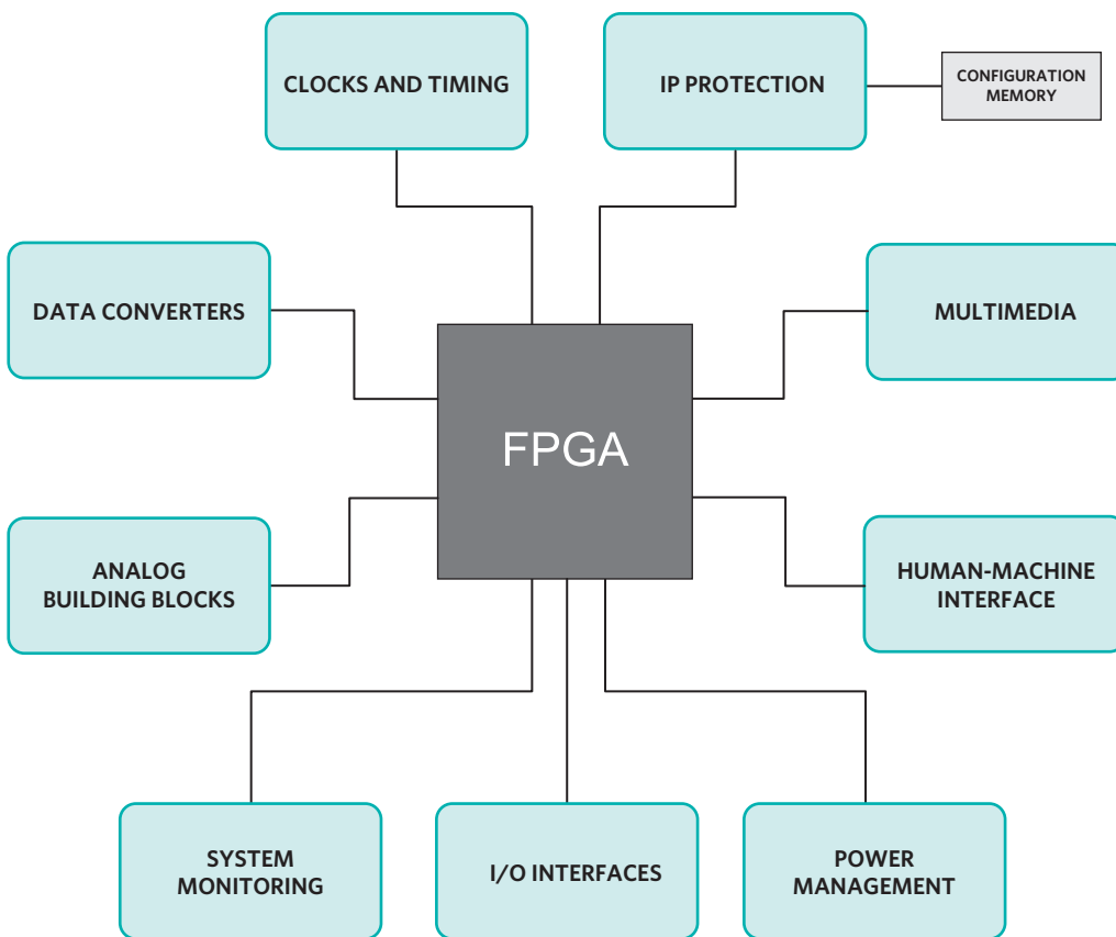
Figure 1. A Typical System Application Showing FPGA Working with Analog Functions
