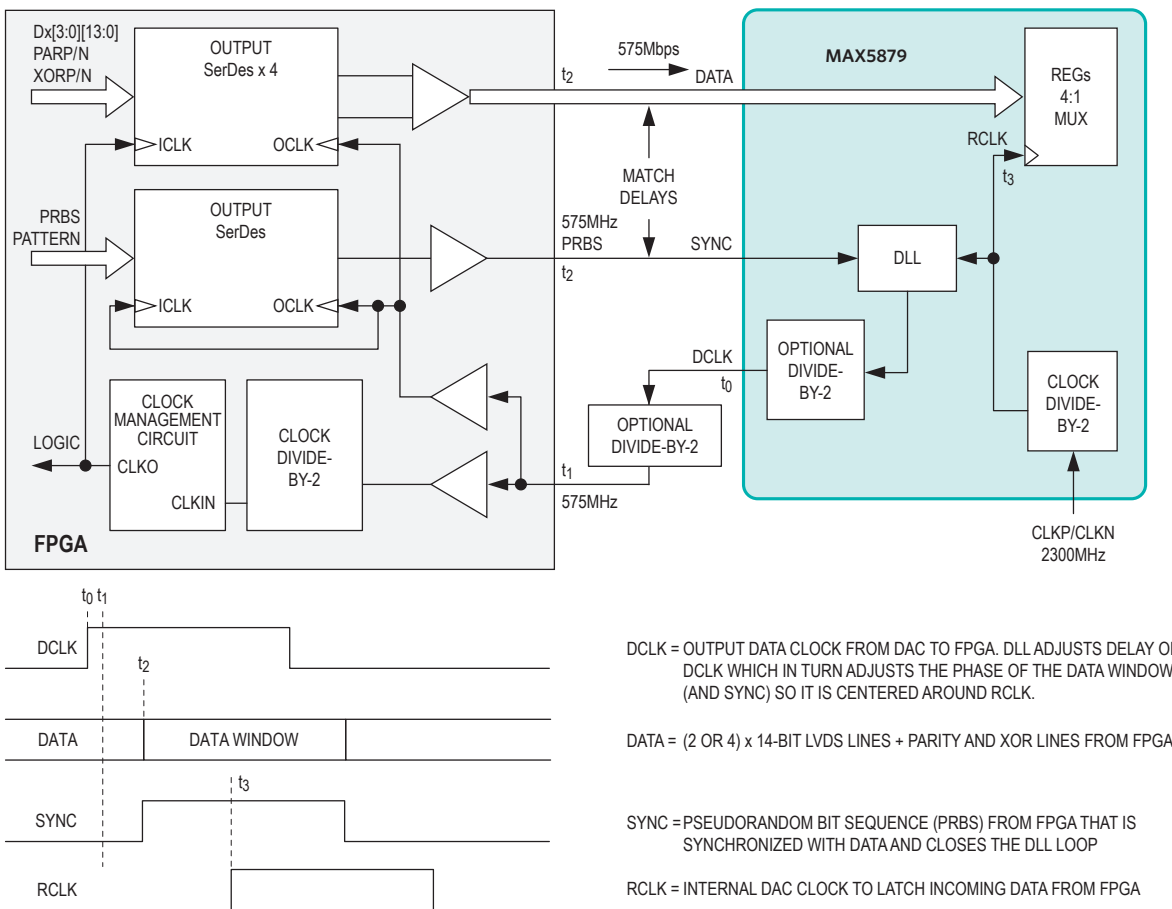
Figure 17. Digital Interface Between the FPGA and the MAX5879 RF-DAC (in 4:1 Mux Mode)
