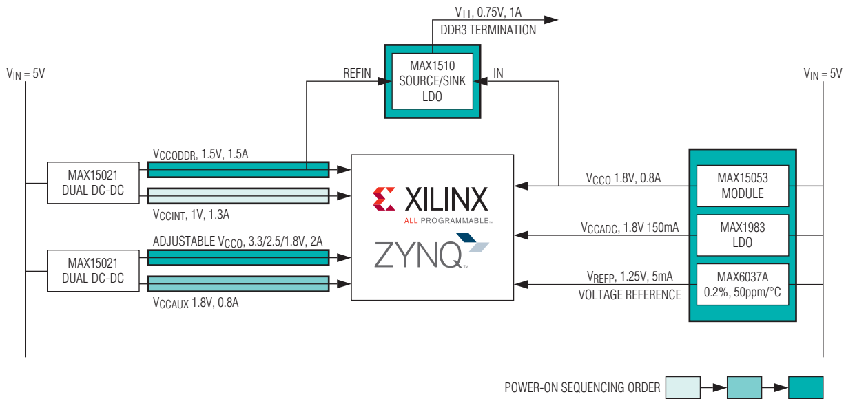
Figure 12. Zynq Extended Processing Platform Power Architecture Example
