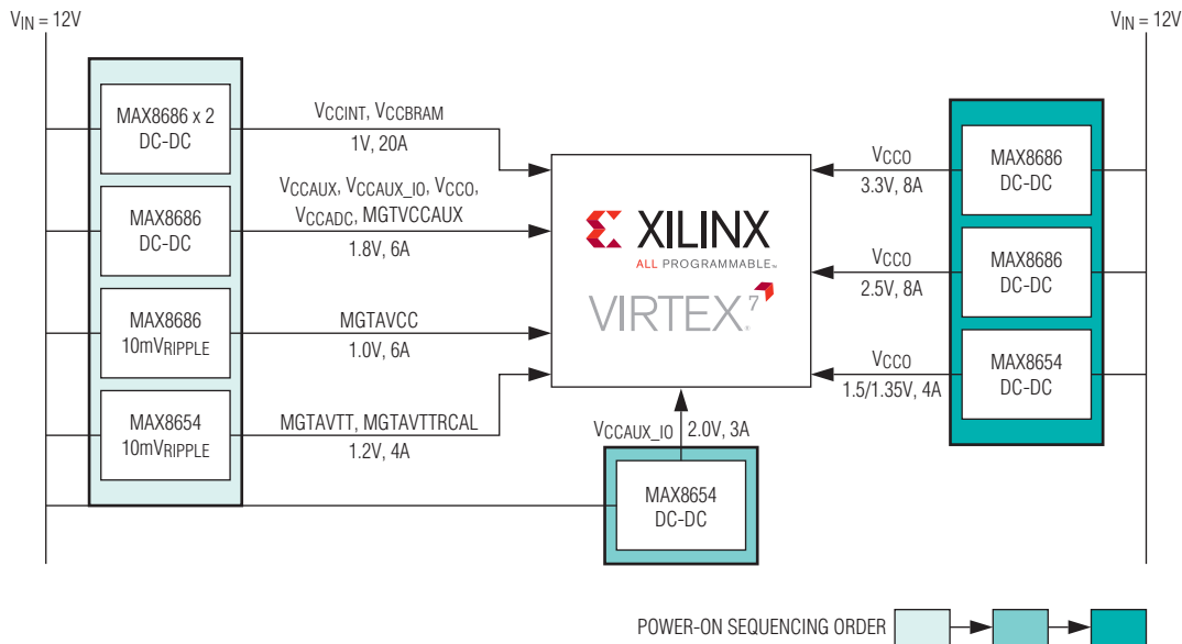
Figure 9. Virtex-7 FPGA Power Architecture Example
