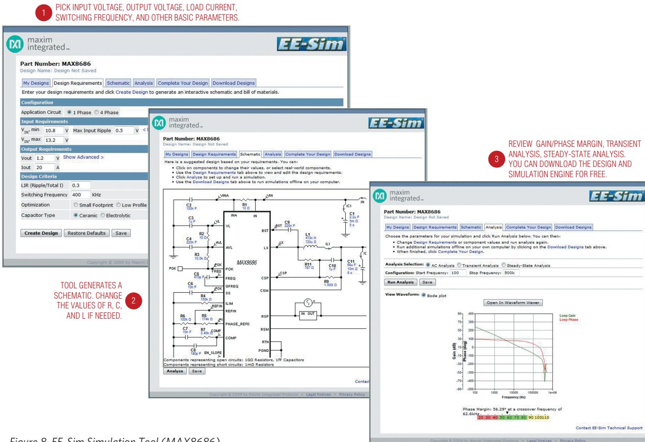
Figure 8. EE-Sim Simulation Tool (MAX8686)
