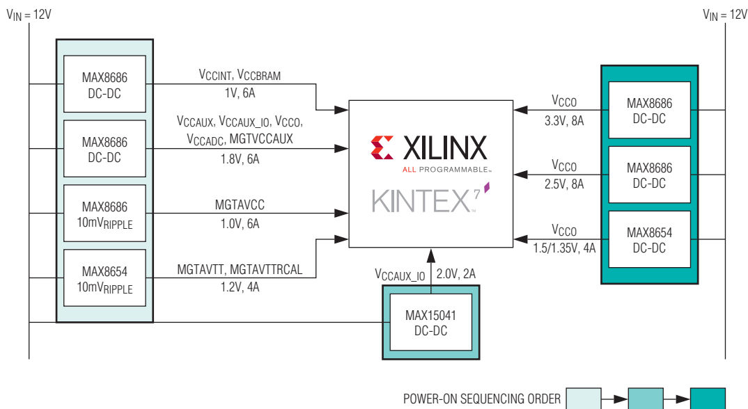
Figure 10. Kintex-7 FPGA Power Architecture Example
