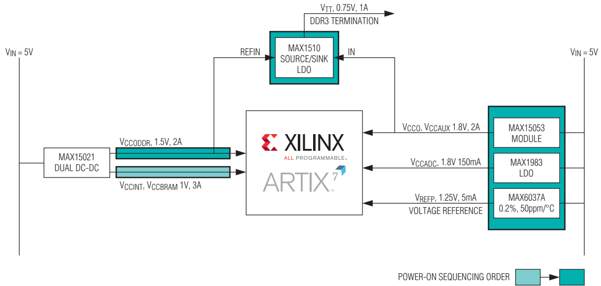
Figure 11. Artix-7 FPGA Power Architecture Example
