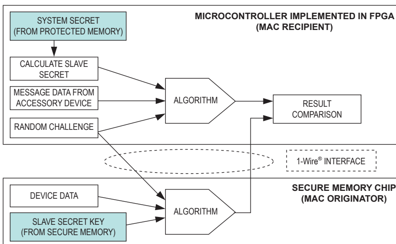
Figure 14. The Challenge-and-Response Authentication Process Proves the Authenticity of a MAC Originator
