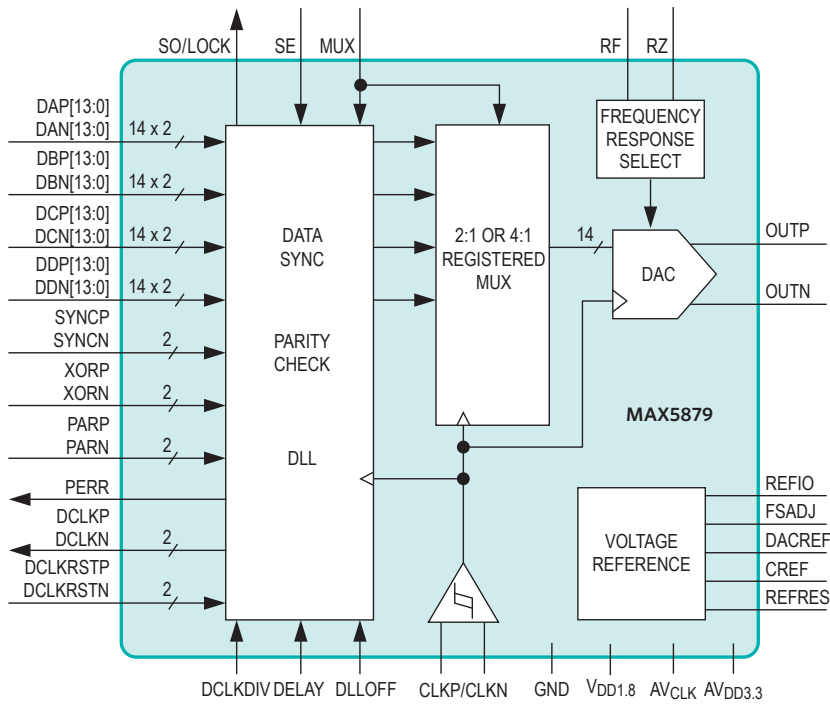
Figure 16. MAX5879 Functional Diagram
