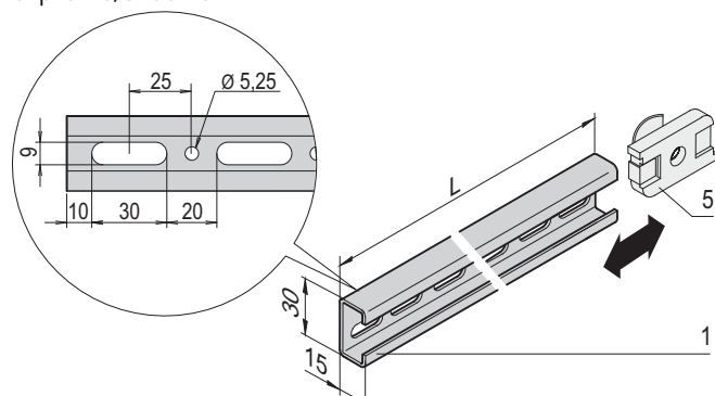
Mounting bracket
