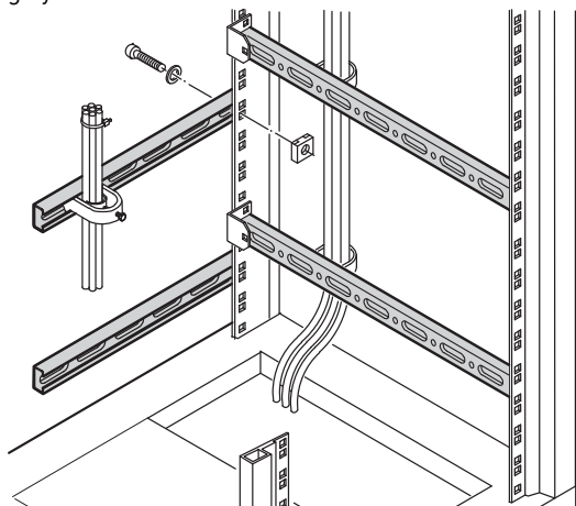
Mounting system
