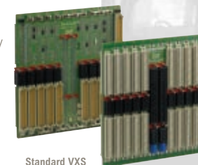
Standard VXS backplanes in a variety of slot counts
