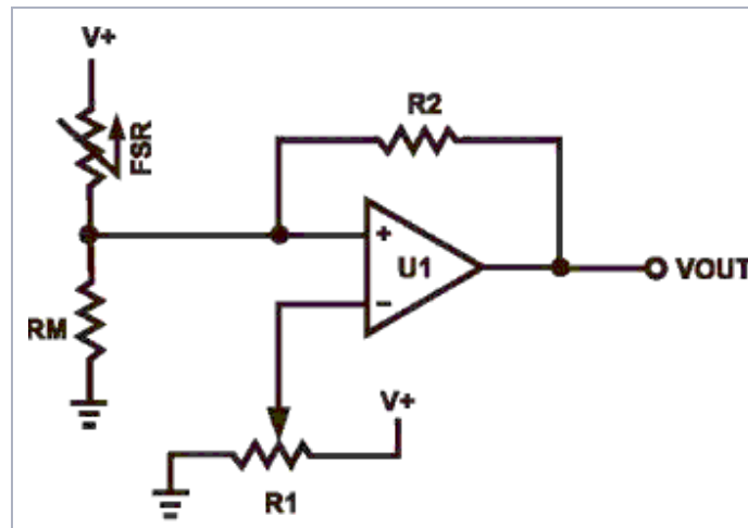
Figure 12: FSR Variable Force Threshold Switch
