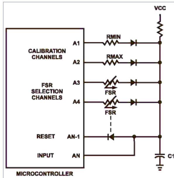
Figure 11: Multi-Channel FSR-to-Digital Interface
