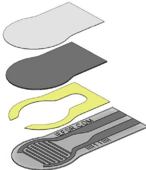
Figure 5: Model 400 Short Tail Round FSR
