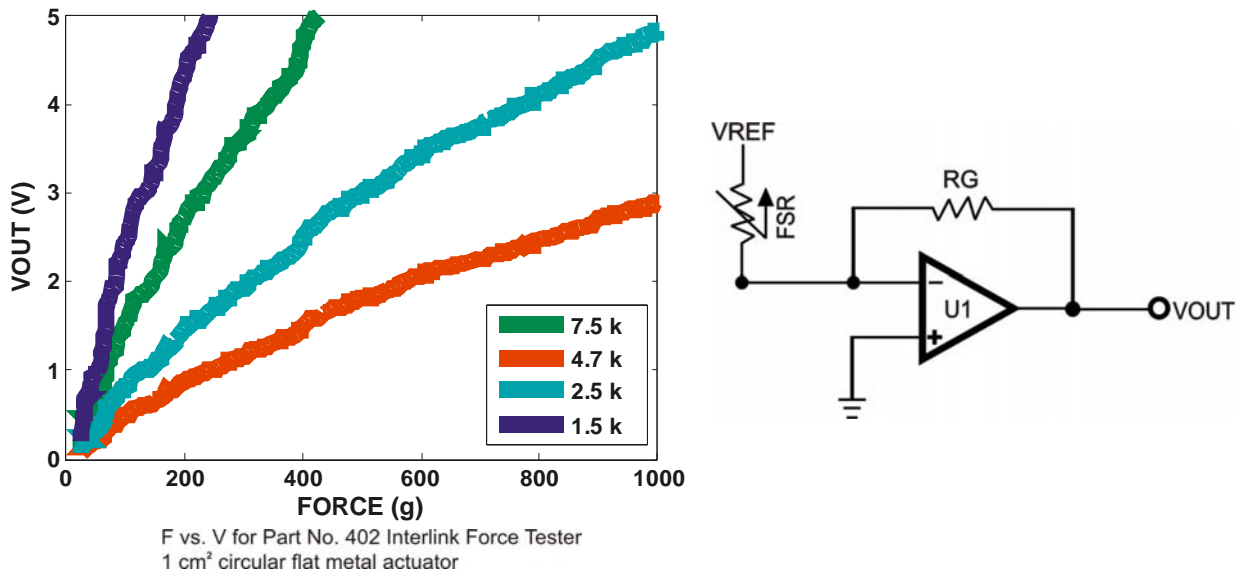
Figure 14: FSR Current-to-Voltage
