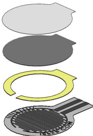
Figure 7: Model 402 Short Tail Round FSR
