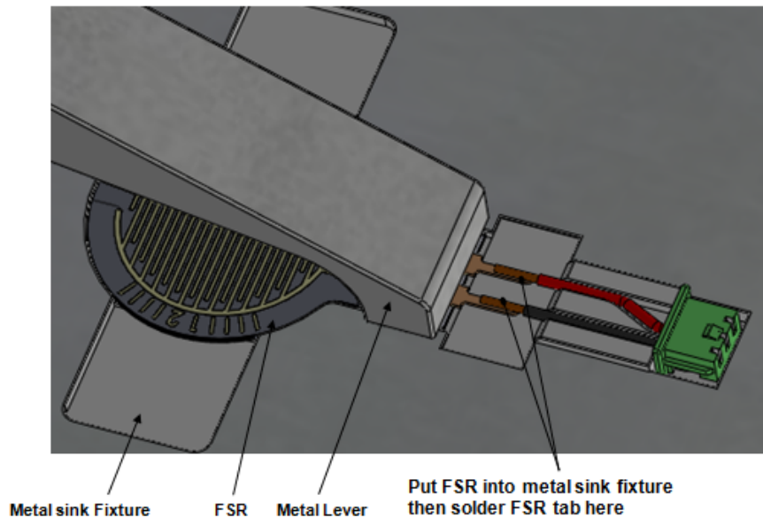
FSR Soldering Fixture
