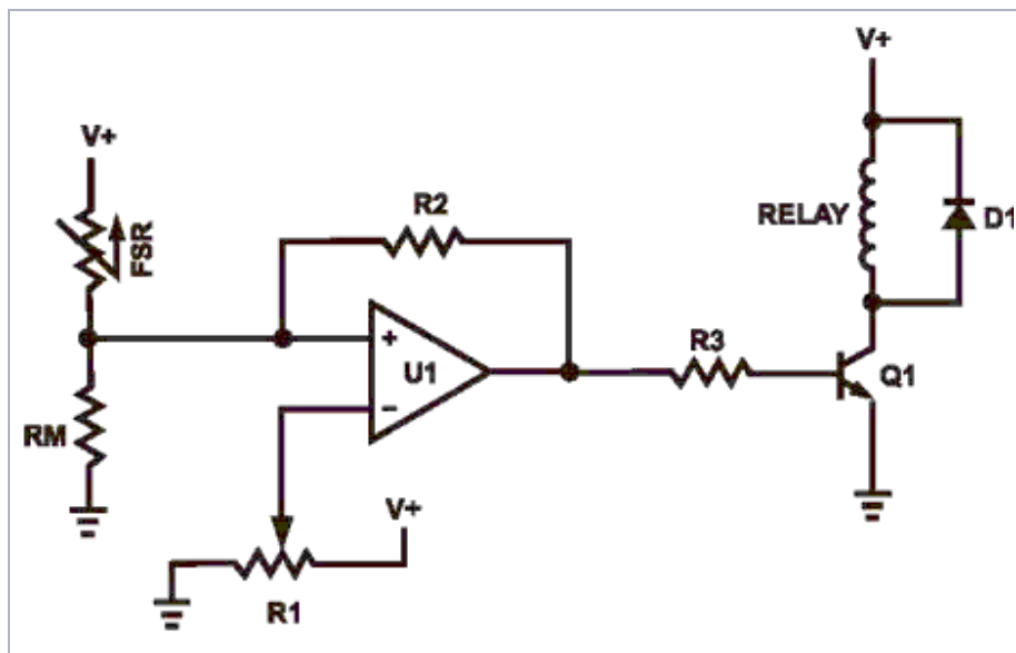
Figure 13: FSR Variable Force Threshold Relay Switch
