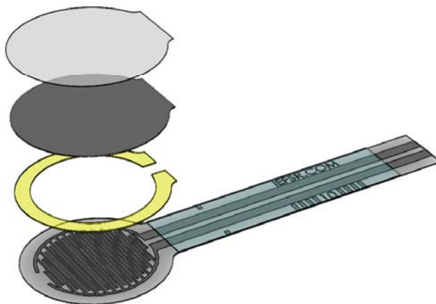
Figure 6: Model 402 Short Tail Round FSR
