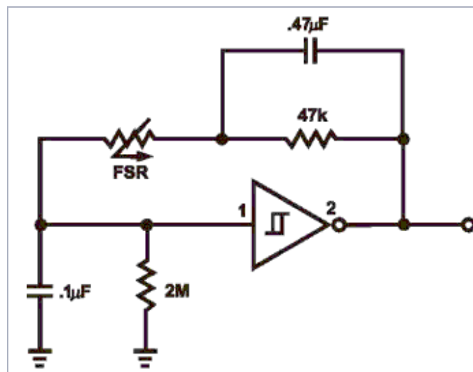
Figure 17: FSR Schmitt Trigger Oscillator
