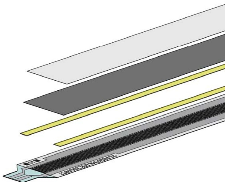
Figure 9: Model 408 Strip FSR
