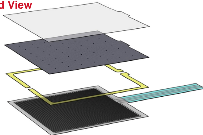
Figure 8: Model 406 Square FSR
