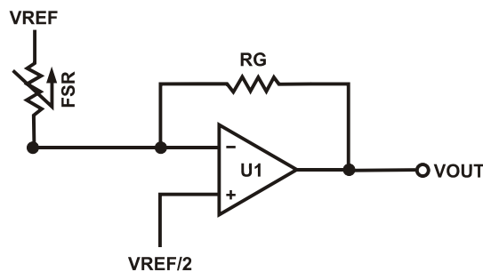
Figure 16: Additional FSR Current-to-Voltage Converter
