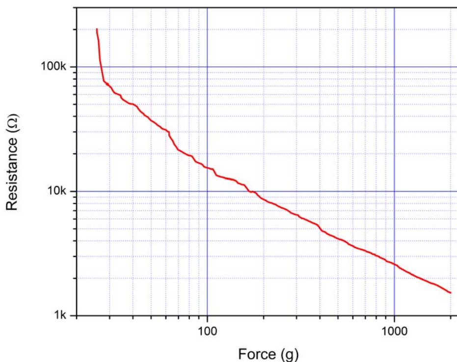
Figure 2: Resistance vs. Force
