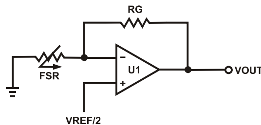
Figure 15: Additional FSR Current-to-Voltage Converter
