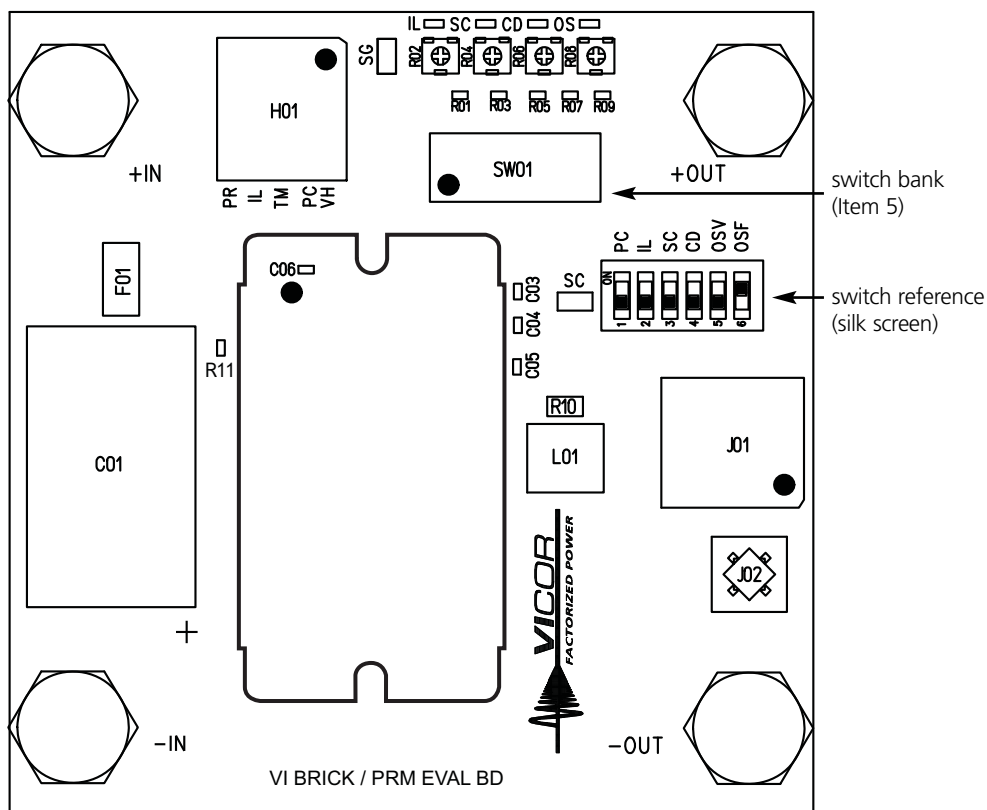
Figure 3 VI BRICK PRM Evaluation Board Layout
