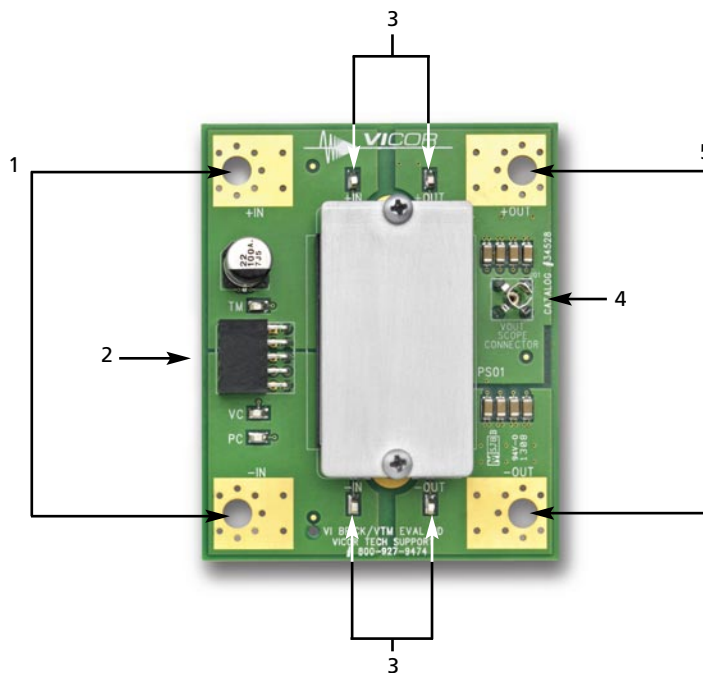
Figure 4 VI BRICK VTM mounted to Evaluation Board
