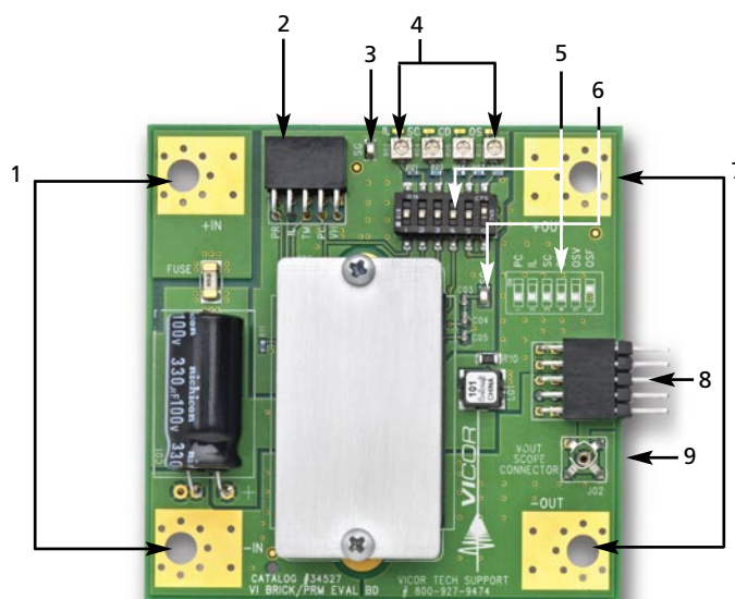
Figure 1 VI BRICK PRM mounted to Evaluation Board
