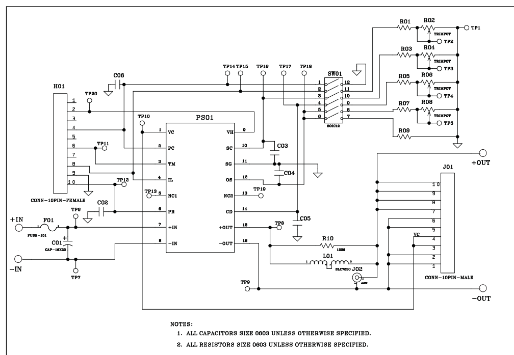
Figure 2 VI BRICK PRM Evaluation Board schematic diagram
