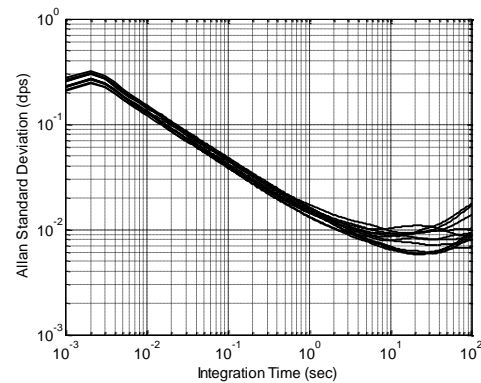
Figure 9: MPU-3000, Allan deviation for 4 units (12 axes)
