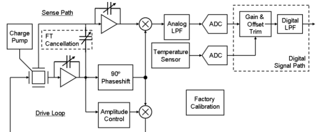
Figure 6: Single-axis gyroscope signal path electronics
