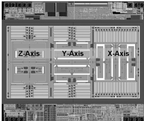
Figure 7: MPU-3000, 3-Axis gyroscope in 2.8mm x 2.4mm
