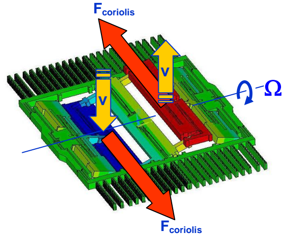
Figure 3: X-axis gyroscope driven mode
