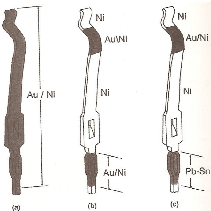
Figure 3. Approaches to plating to reduce gold without decreasing performance.
