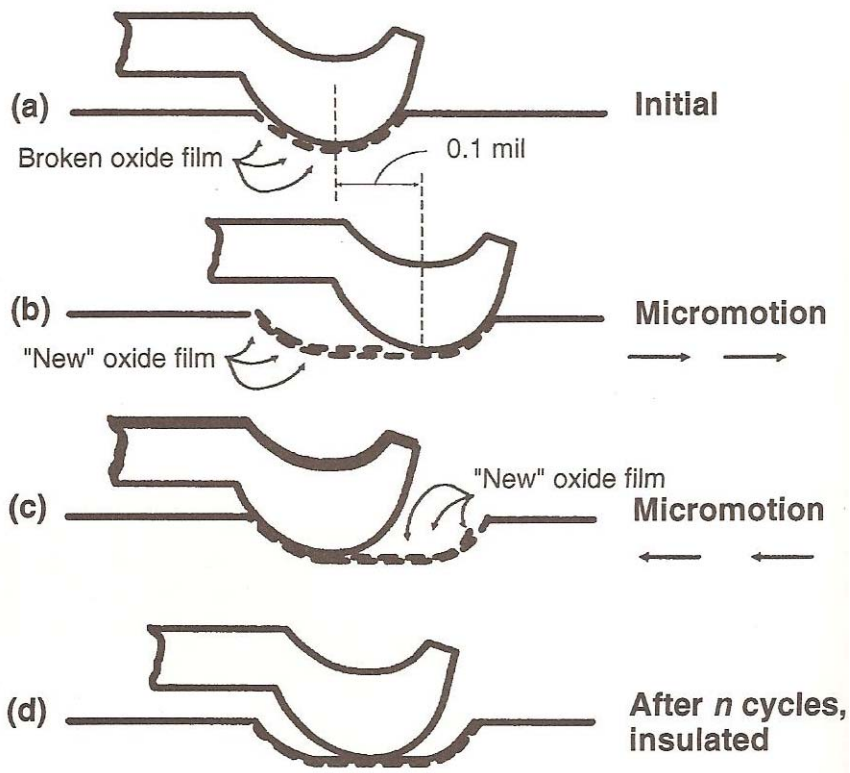
Figure 5. Fretting corrosion from micromotions
