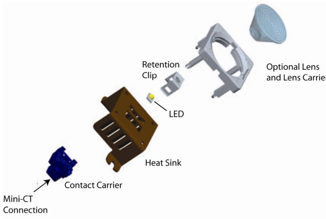
Figure 7. High-intensity LED holder combines thermal, mechanical, and electrical management into a single, easy-to-use system.
