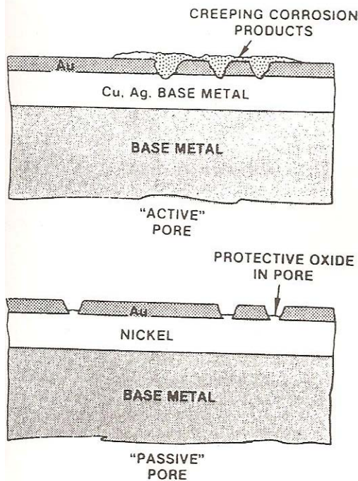
Figure 4. Nickel prevents corrosion from migrating through micropores from the base material through gold plating to the surface.
