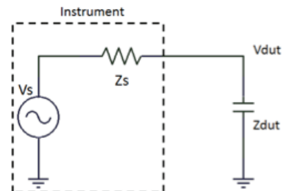
Figure 1. Schematic of Capacitance Measurement with Source Impedance
