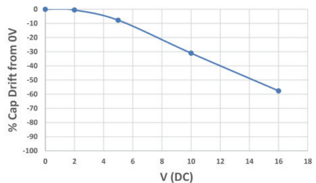
Figure 6. Capacitance versus DC Voltage
