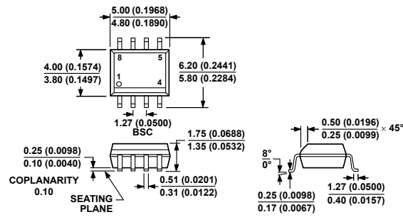
Figure 67. 8-Lead Standard Small Outline Package [SOIC_N] Narrow Body (R-8)
