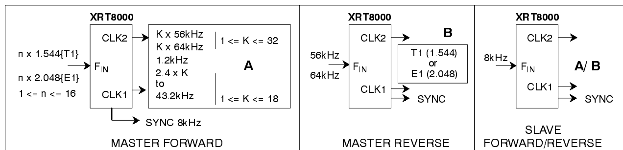
Figure 1. System Diagram
