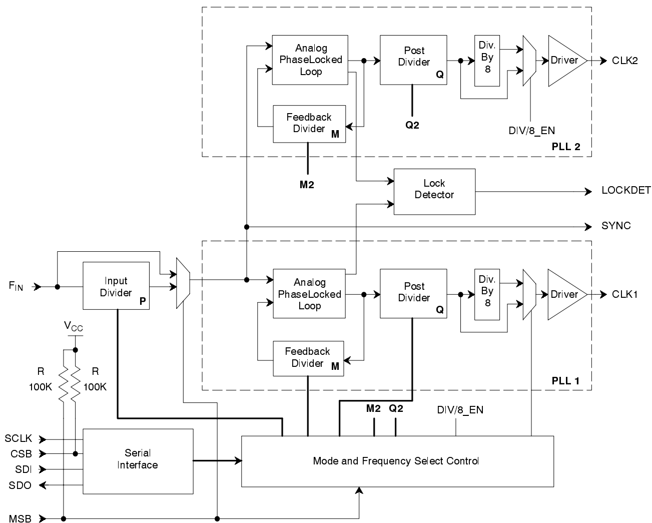
Figure 2. Block Diagram
