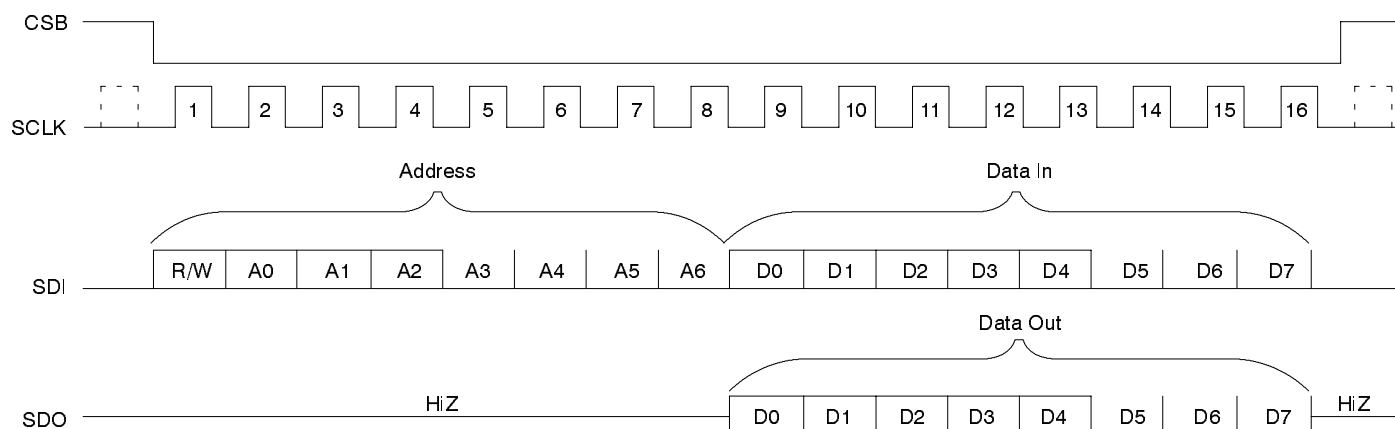
Figure 4. Serial Processor Interface Data Structure
